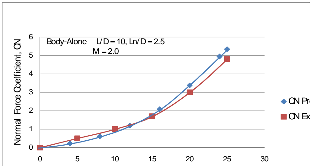
Figure 10: Comparison of program output with experiment for body-alone at M = 2.0
