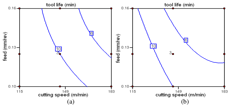
Figure 4: Response surface graphs of contours for tool life of (a) conventional and (b) wiper tools
