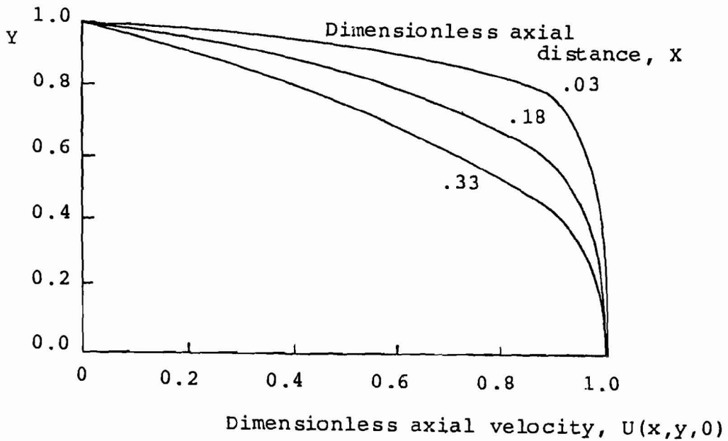
Figure 6 Axial velocity profiles on center plane Z = 0
