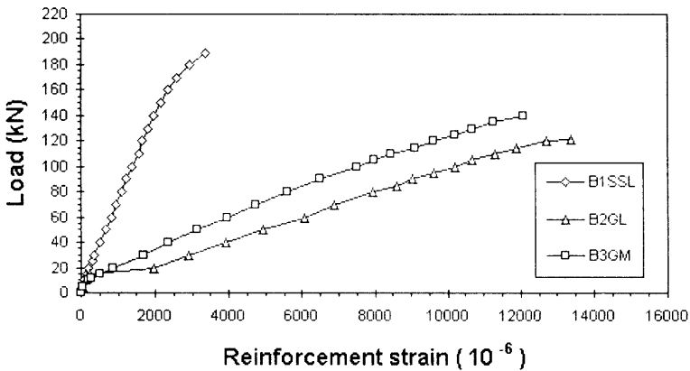
Figure 4: Load-reinforcement strain for all beams tested
