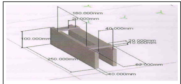
Figure 10: Blade
