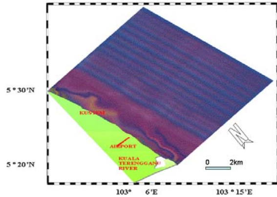
Fig.2. Holographic fringes for wave refraction pattern.
