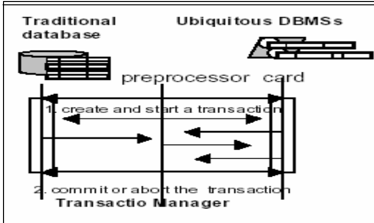
Figure 2.2 : 2-phases commitment
