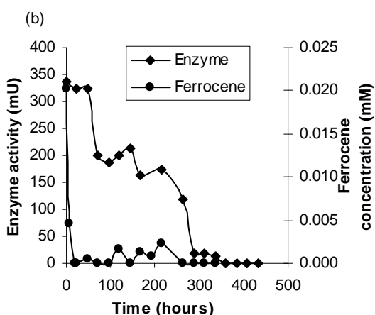
Figure 1. Leaking profile for CLPVA-GOD/Fc membrane with different GOD and BSA loading a) 1:1 b) 1:3 (weight ratio of GOD: BSA).
