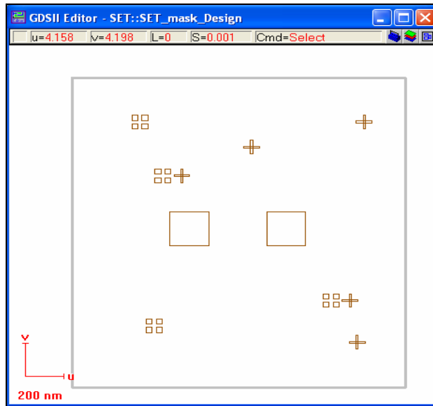
Fig. 5: Contact mask.
