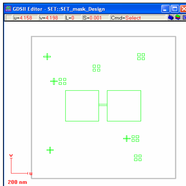
Fig. 3: The source and drain mask.
