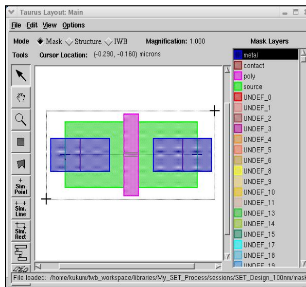
Fig. 9: Mask layout for SET simulation designed using Taurus Layout.
