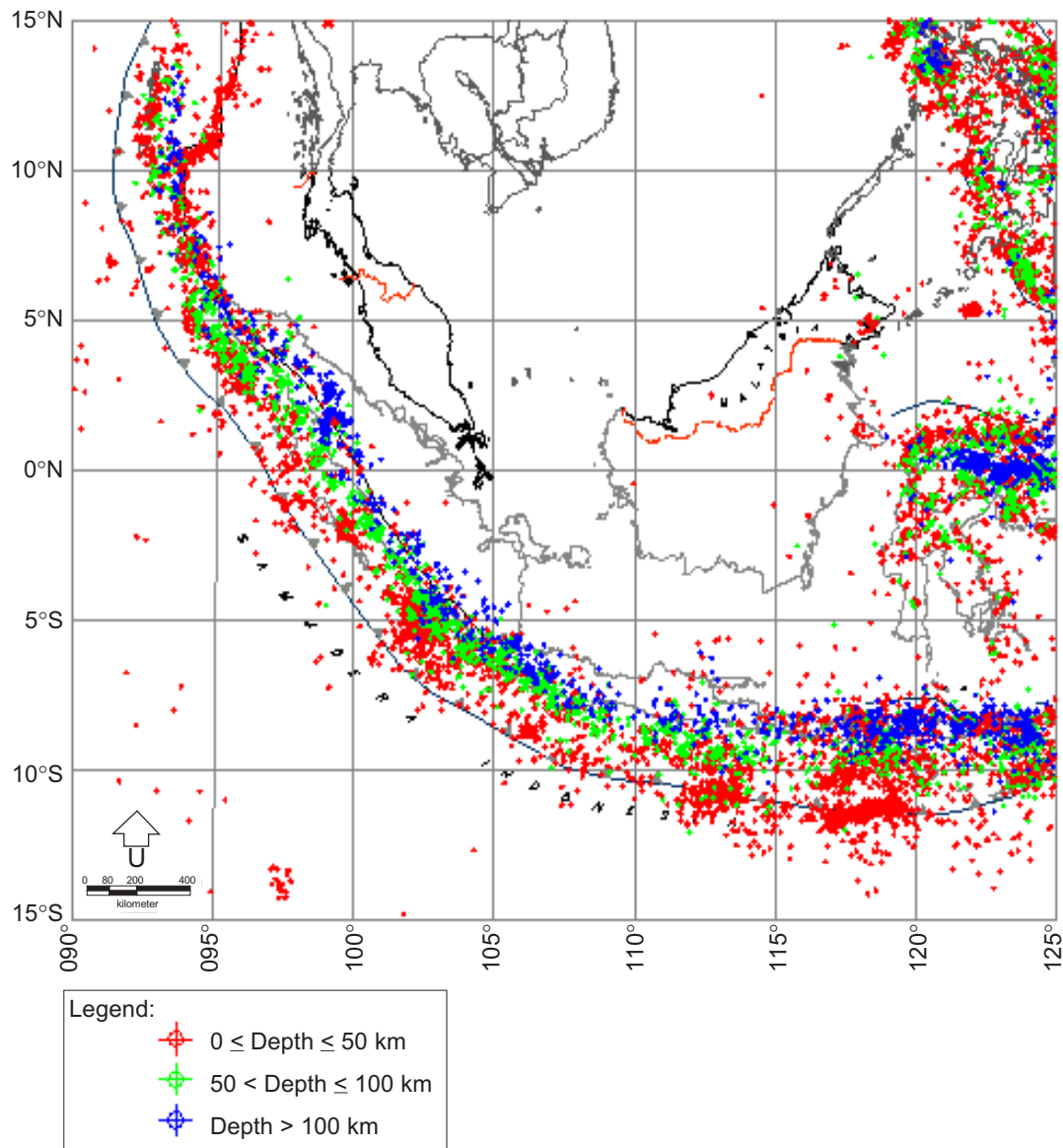
Figure 1 Historical earthquakes around Peninsular Malaysia ( M_w > 5.0 )
