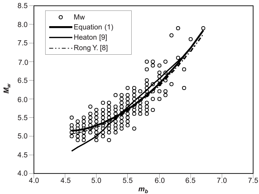
Figure 4 The relationship between m_b and M_w
