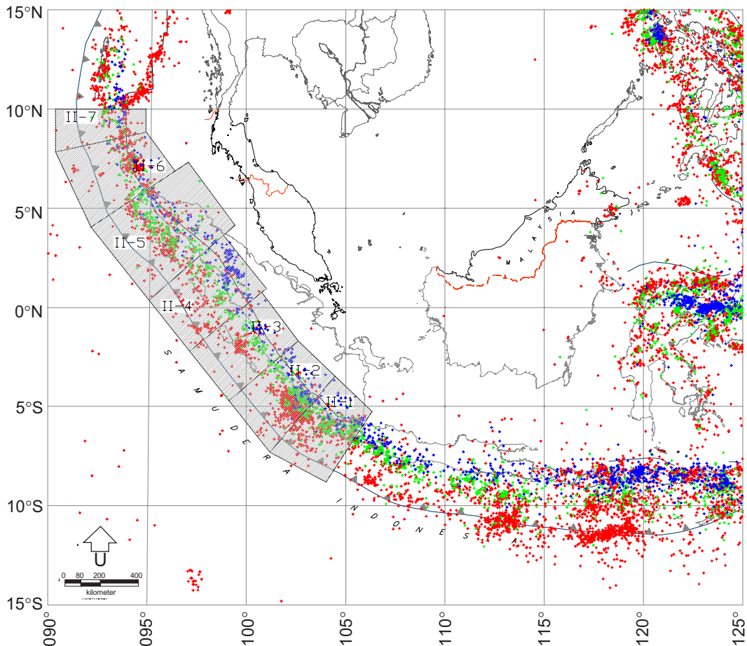
Figure 7 Seismic source zones around Peninsular Malaysia
