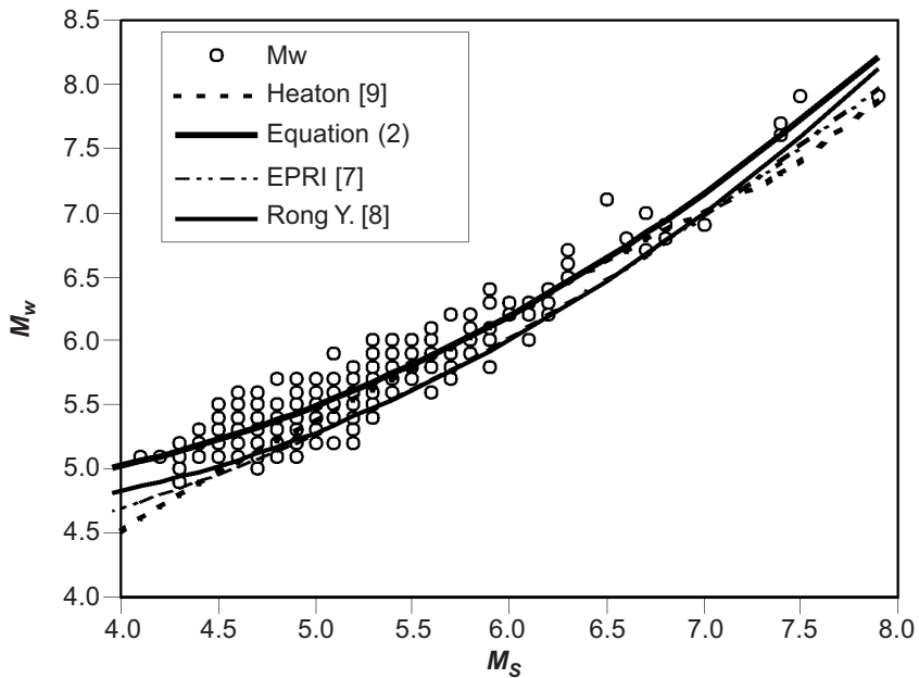
Figure 5 The relationship between M_s and M_w
