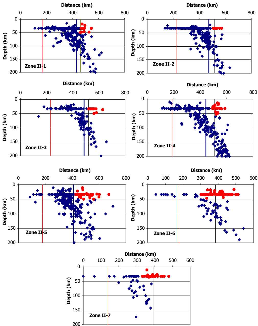
Figure 8 Hypocentral profiles
