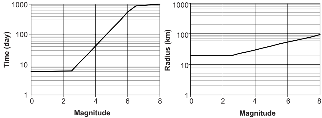
Figure 6 Time and distance windows
