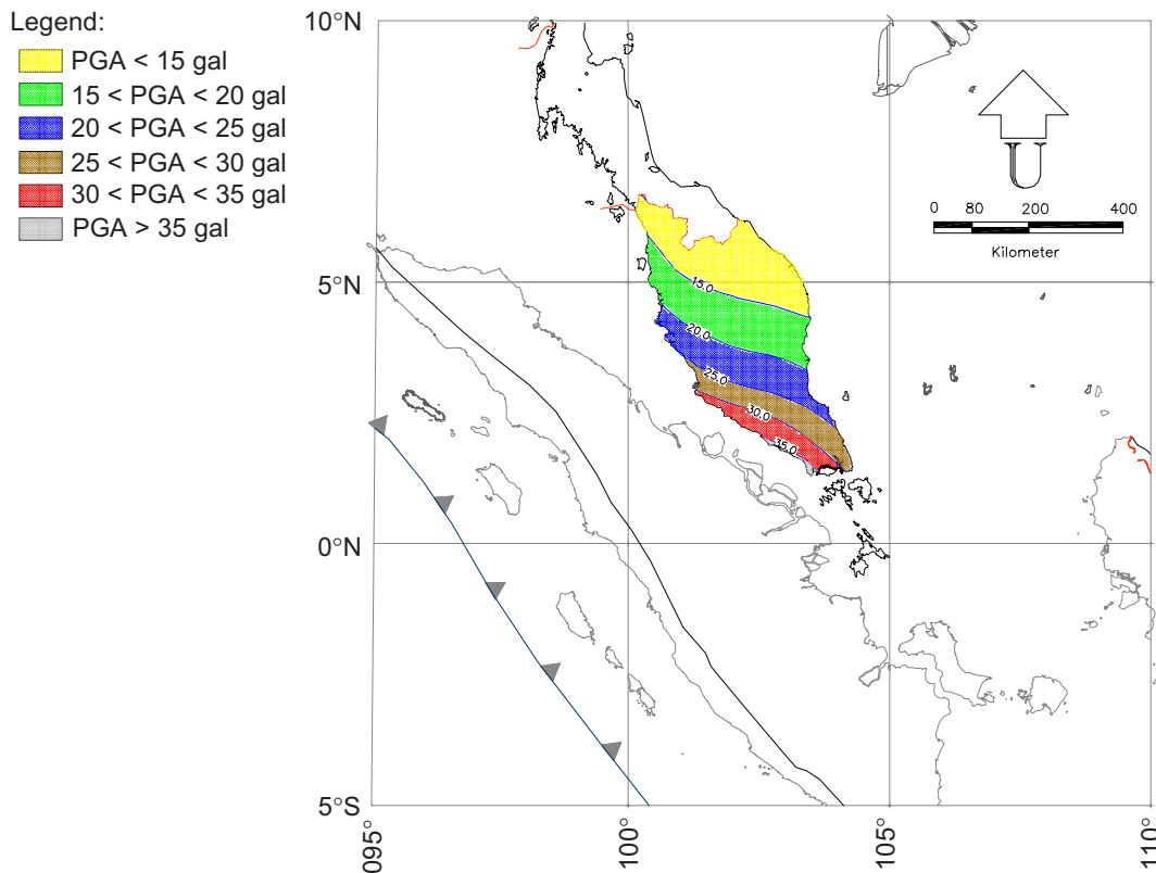
Figure 10 PGA with 2% probability of exceedance in 50 years
