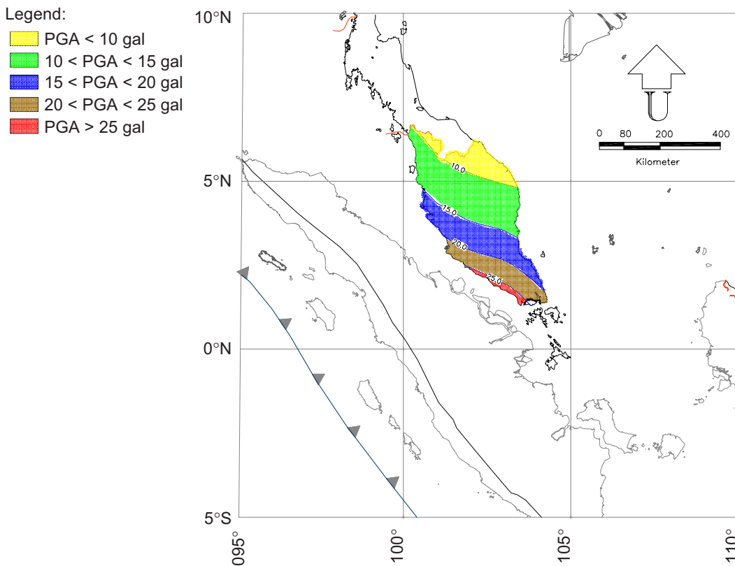
Figure 9 PGA with 10% probability of exceedance in 50 years
