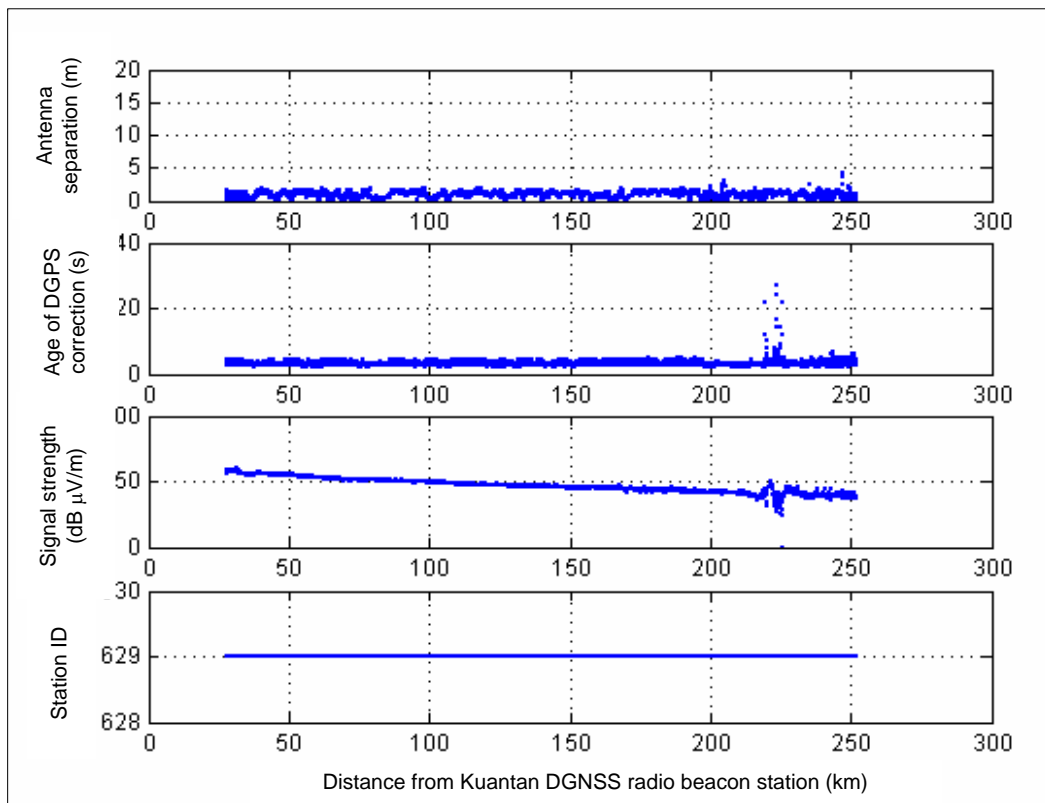
Figure 12: Result for manual tracking method (dynamic test)
