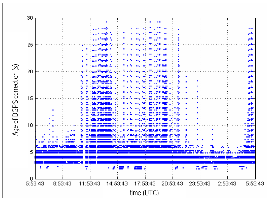
Figure 6: Age of DGPS correction at 250 kilometres distance
