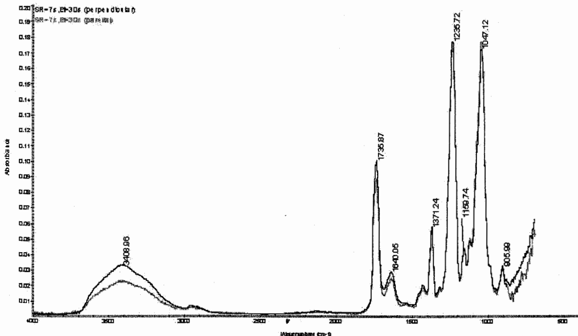
Figure 4. Polarized reflection IR spectra of the NF membranes at shear rates of 217.14s^{-1} . The plane of polarization of the IR beam was parallel (lighter line) and perpendicular (darker line) to the shear direction
