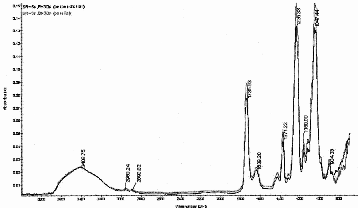
Figure 5. Polarized reflection IR spectra of the NF membranes at shear rates of 304.00s -1 . The plane of polarization of the IR beam was parallel (lighter line) and perpendicular (darker line) to the shear direction
