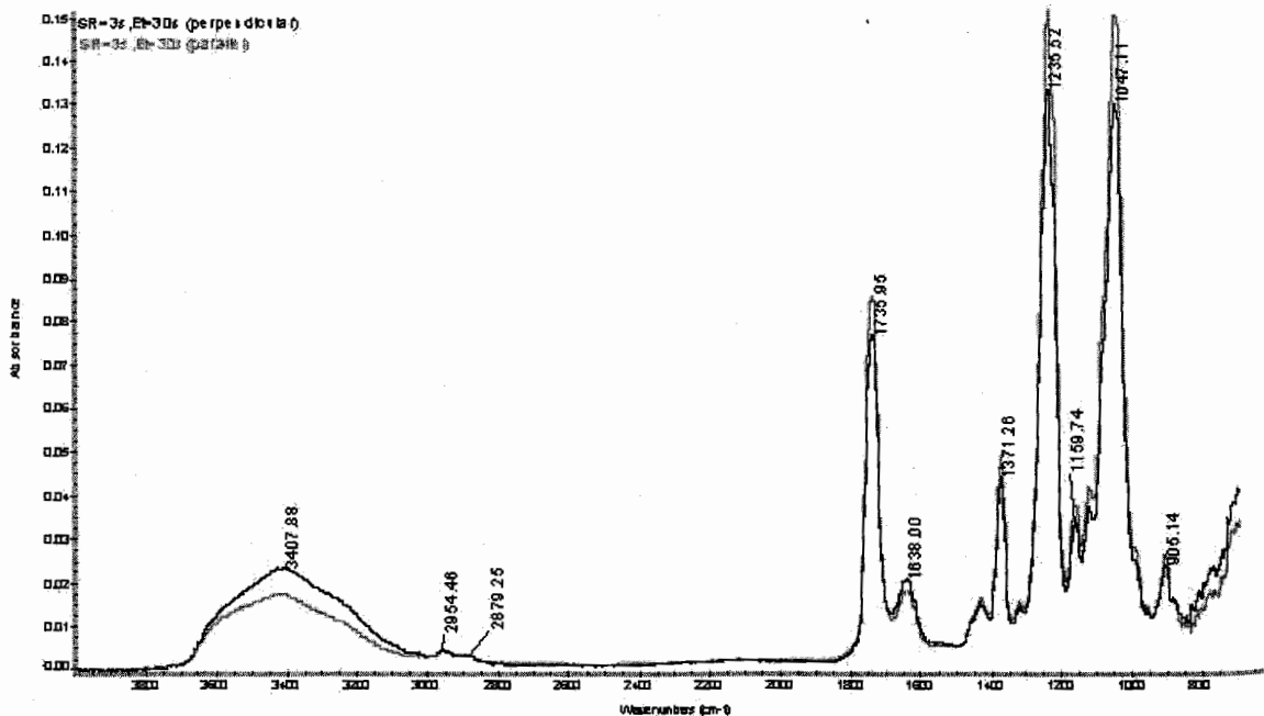
Figure 6. Polarized reflection IR spectra of the NF membranes at shear rates of 506.67s -1 . The plane of polarization of the IR beam was parallel (lighter line) and perpendicular (darker line) to the shear direction
