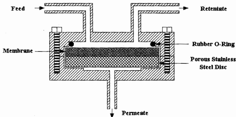
Figure 1. Permeation cell
