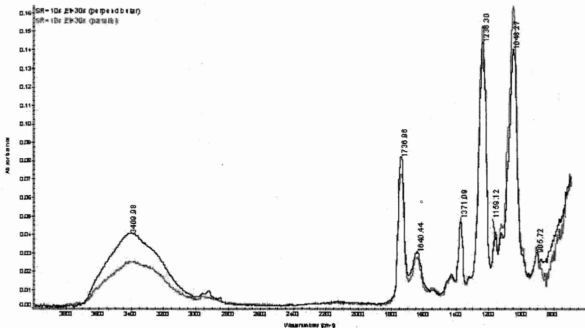
Figure 3. Polarized reflection IR spectra of the NF membranes at shear rates of 152.00s^{-1} . The plane of polarization of the IR beam was parallel (lighter line) and perpendicular (darker line) to the shear direction
