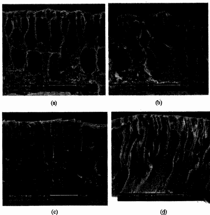
Figure 7. SEM of cross-section of NF membranes at different shear rates; (a) 152\text{ s}^{-1} , (b) 217\text{ s}^{-1} , (c) 304\text{ s}^{-1} , (d) 507\text{ s}^{-1}
