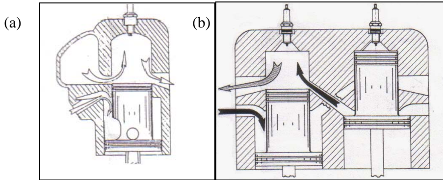
Figure 1: (a) Single-cylinder and (b) multi-cylinder arrangements [2].
