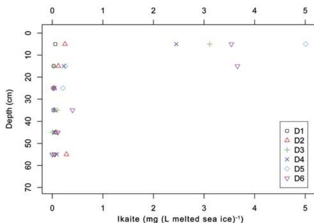
Fig. 6. Distribution of ikaite in sea ice during Dumont d’Urville campaign in land fast sea ice off Terre Adélie sampled in November 2007.
