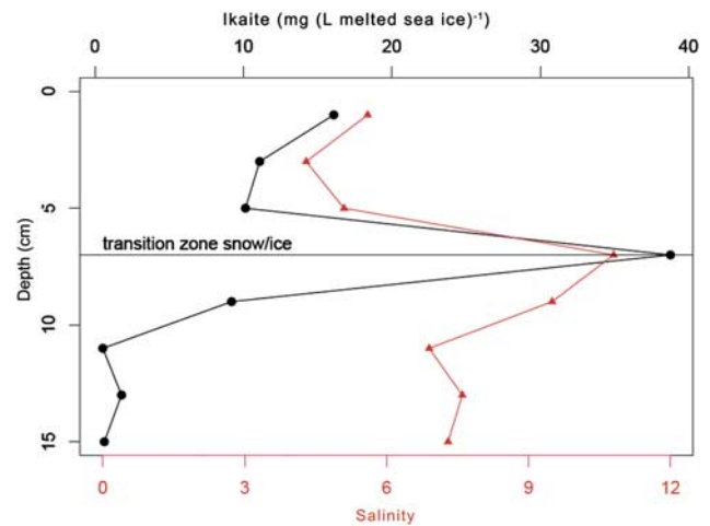
Fig. 9. Distribution of ikaite across the snow-ice interface from top layer of land fast sea ice off Terre Adélie (Dumont d'Urville) in November 2007, core D8. Black line = amount of ikaite, red line = bulk salinity, in contrast to the general use of the 0 cm for the snow/ice interface, here it indicates the top of the snow.
