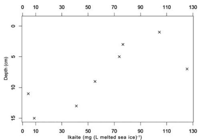
Fig. 8. Distribution of ikaite in the top layer of older (one year) land fast sea ice, off Terre Adélie (Dumont d'Urville) in November 2007 core D10.
