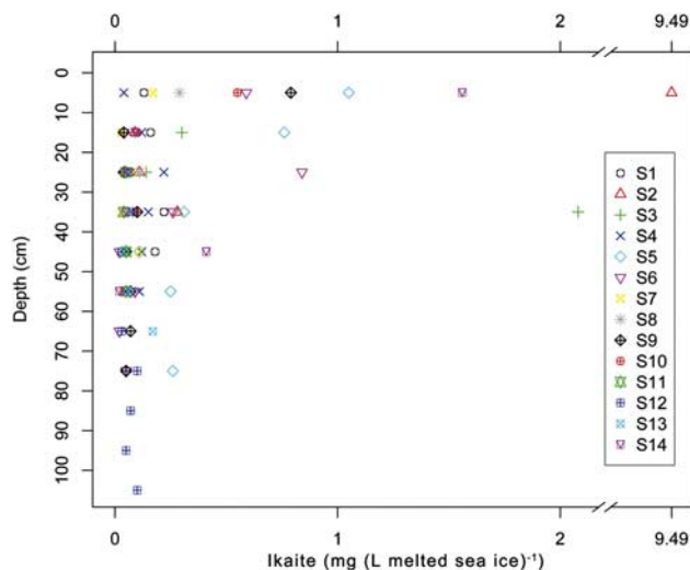
Fig. 5. Distribution of ikaite in sea ice during SIPEX cruise in different ice cores taken between September and October 2007 in East Antarctic.
