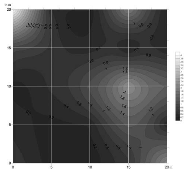
Fig. 10. Contour plot of the spatial distribution of ikaite in the upper 10 cm of land fast sea ice off Terre Adélie (Dumont d'Urville) in November 2007 on a 20 m x 20 m grid with sample points every 5 m x 5 m (shown by intersections of the white lines and at the edges). Values are in mg ikaite l -1 melted sea ice.
