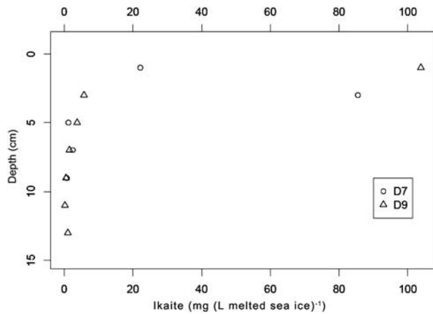
Fig. 7. Distribution of ikaite in the surface layer of young (three month) land fast sea ice off Terre Adélie (Dumont d'Urville).
