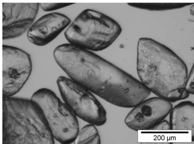
Fig. 4. Light microscopy image of ikaite crystals taken from a single bulk sea ice sample from land fast ice off Terre Adélie.
