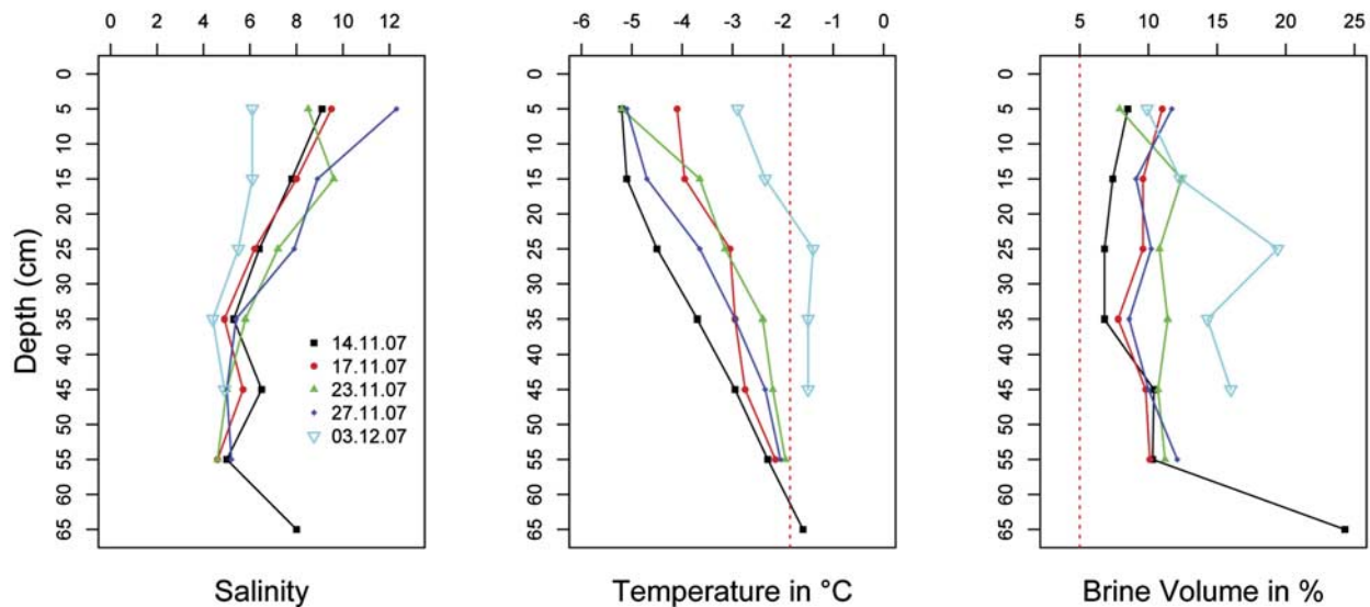
Fig. 3. Bulk salinity, sea ice temperature, and calculated (Cox & Weeks 1986) brine volume in land fast sea ice cores taken between November and December 2007 in East Antarctic during Dumont d'Urville campaign.
