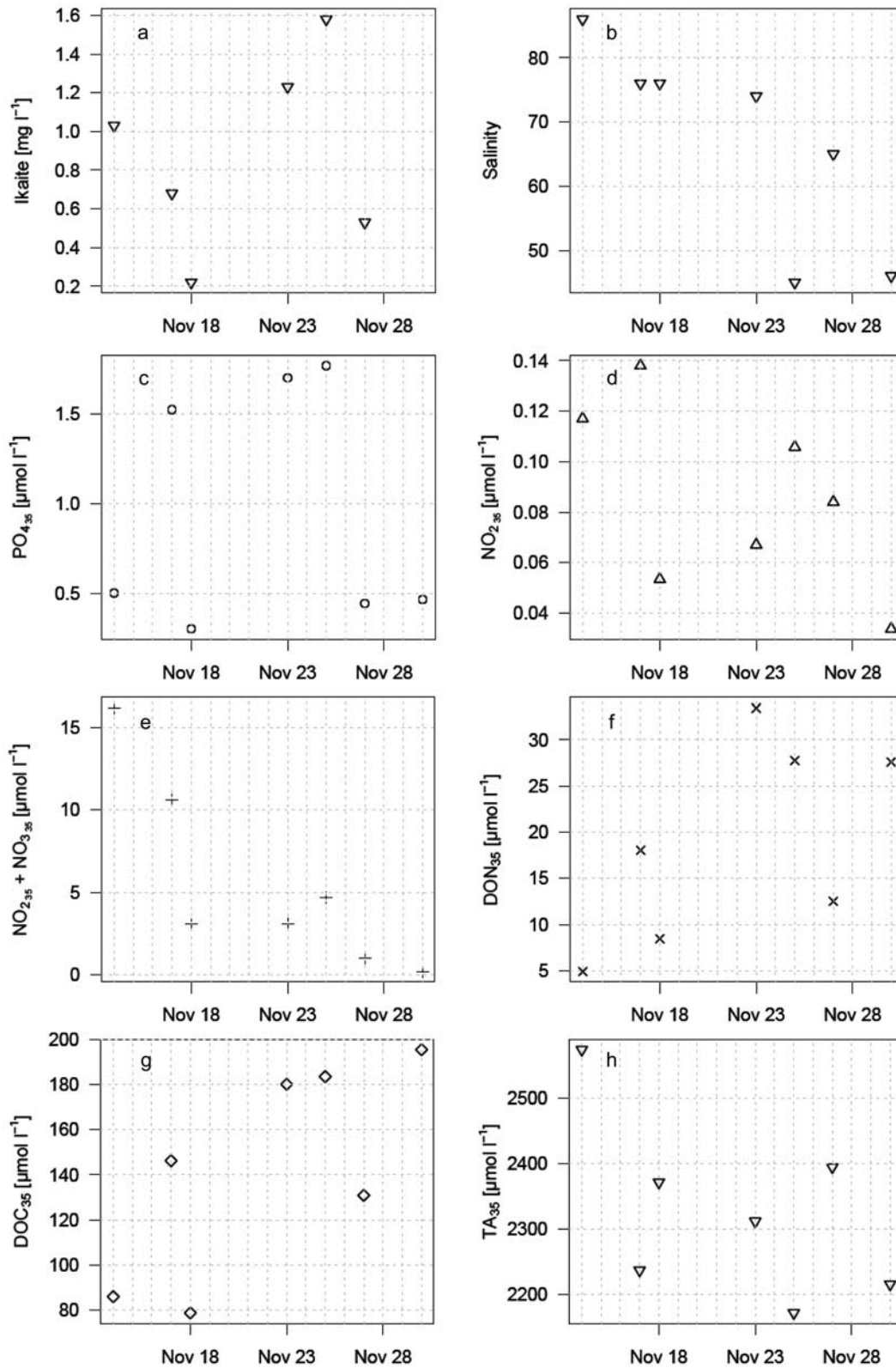
Fig. 11. a. Temporal observation of ikaite in ice cores (30 cm) obtained from sackholes D-SH1 to D-SH7 (Dumont d'Urville (DDU) campaign), b. salinity, c. salinity-normalized \text{PO}_4^{2-} , d. \text{NO}_2^- , e. (\text{NO}_2) + (\text{NO}_3)_{35} , f. dissolved organic nitrogen (DON), g. dissolved organic carbon (DOC), and h. total alkalinity (TA) in Antarctic land fast sea ice, off Terre Adélie (DDU) in November 2007.
