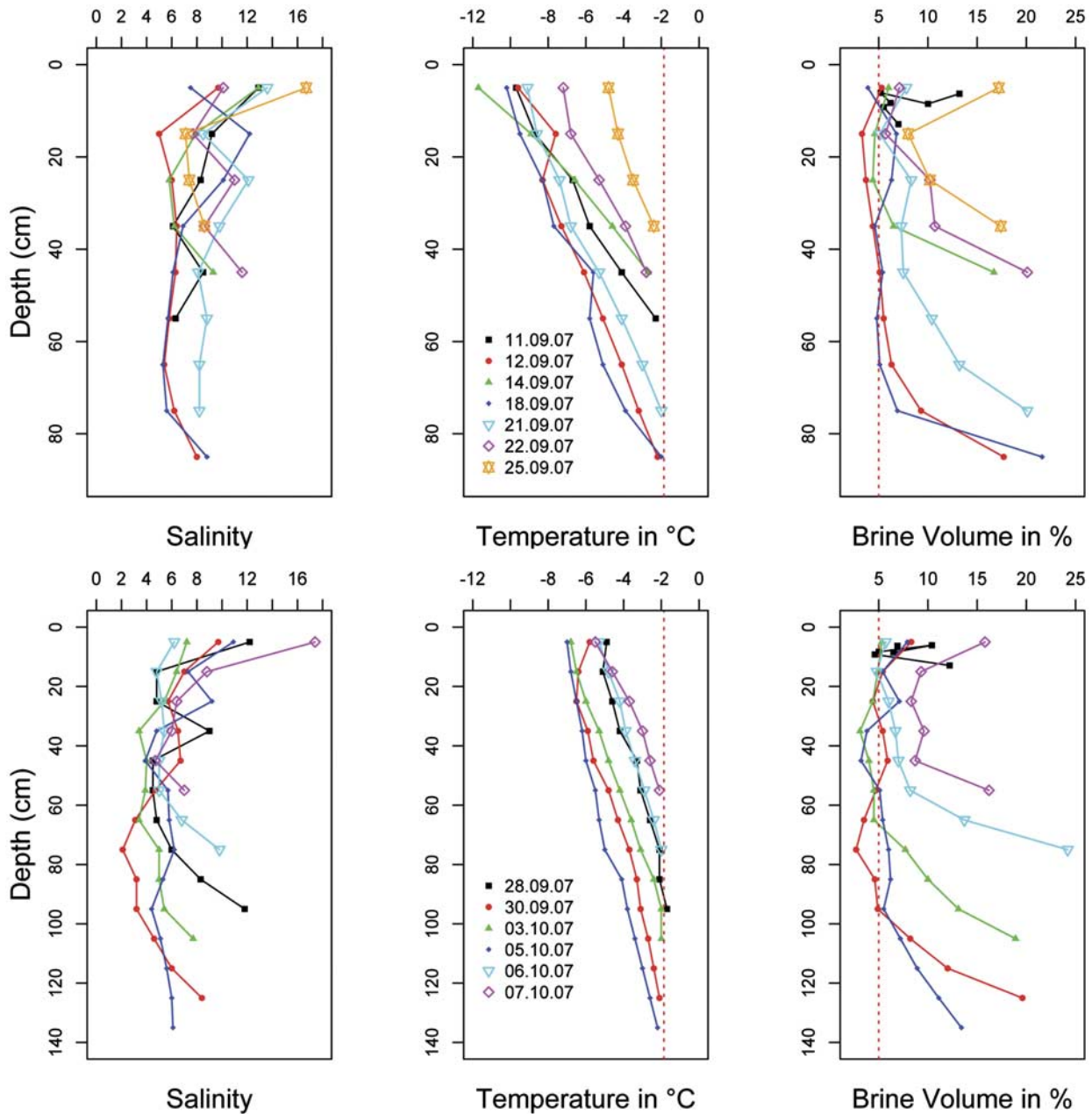
Fig. 2. Bulk salinity, sea ice temperature, and calculated (Cox & Weeks 1986) brine volume in different ice cores taken between September and October 2007 in East Antarctic during SIPEX campaign.
