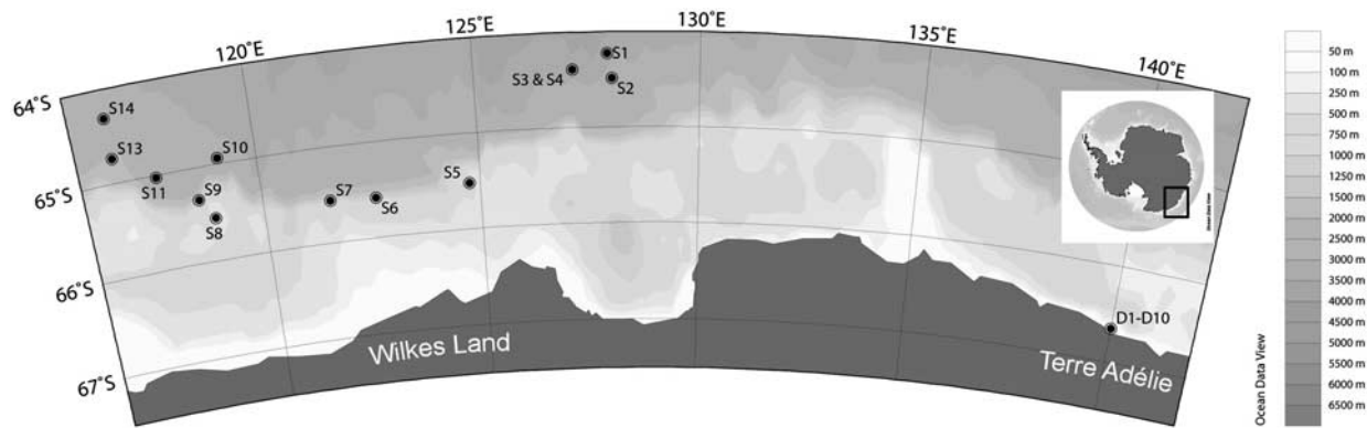
Fig. 1. Locations of ice stations sampled during Sea Ice Physics and Ecosystem eXperiment (SIPEX) and Dumont d'Urville (DDU) campaigns.
