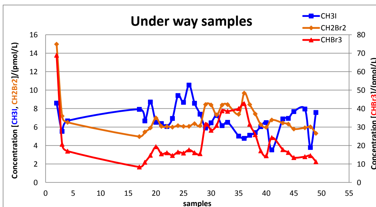
Figure 1: Preliminary concentration of methyl iodide, dibromomethane and bromoform in the under way samples.
