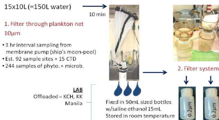
Figure 1: Schematic of sampling method employed on RV Sonne SO218. This includes filtration of estimated 150L of seawater through a 10 µm plankton net, and further filtration using filtration system then stored in 50 mL screw cap bottles with 15 mL saline ethanol at room temperature. Samples come offboard the RV Sonne in Kuching (KCH), Kota Kinabalu (KK) and Manila.
