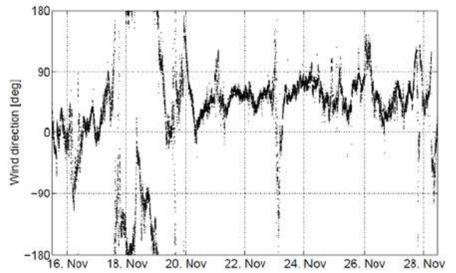
Figure 2: Ship measurements of wind speed (m/s), wind direction (degree E) and surface air temperature (°C).
