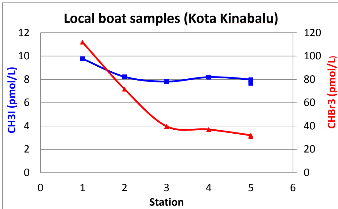
Figure 2: The local boat samples by Kota Kinabalu (preliminary concentrations).
