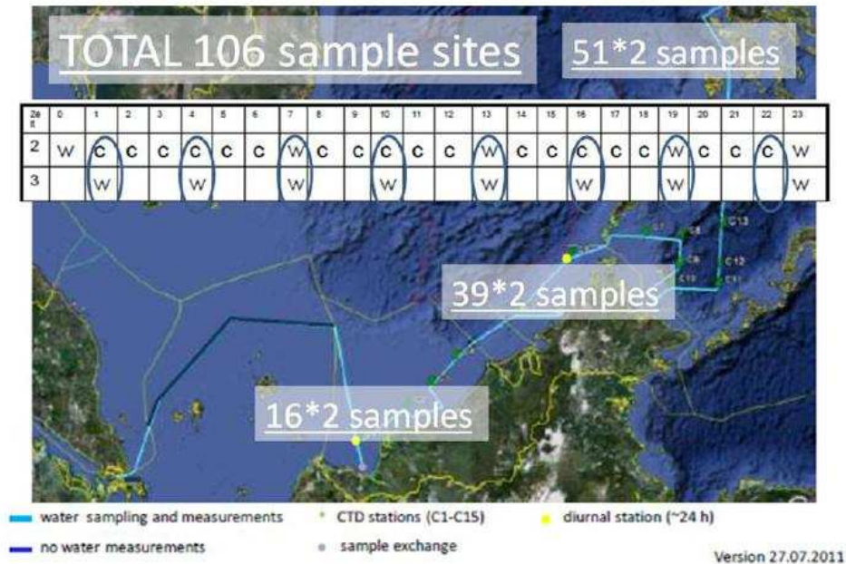
Figure 2: Map of sampling cruise track of the RV Sonne SO218. The 24 hour operation would sample water (marked w) every 3-hourly, starting at 0100 everyday. A total number of 106 sites in the SCS have been sampled, with underway 3 hourly sampling bottles of 32 (phytoplankton and microbial) samples come offboard the RV Sonne at Kuching (KCH), 78 samples offboard in Kota Kinabalu (KK) and 102 samples offboard in Manila. The rest of live samples and CTD samples are taken from Manila to Kuching.
