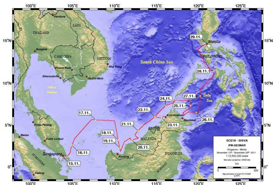
Figure 1: Cruise track of RV Sonne: Singapore-Manila (15-29 November 2011).
