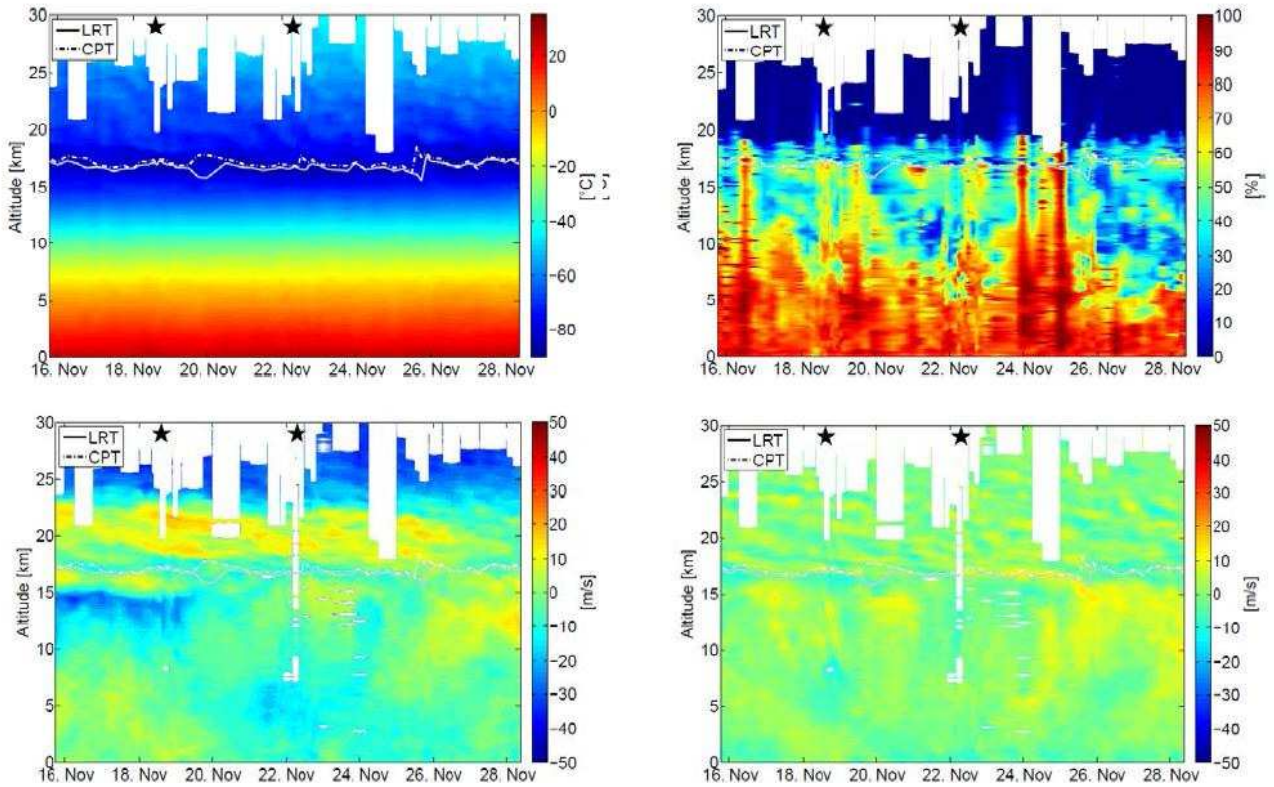
Figure 1: Profiles obtained from the radio sounding: Left: Temperature ( ^{\circ}\text{C} ), the dashed line shows the cold point temperature (CPT) and the solid line displays the lapse rate temperature (LRT); Right: Relative humidity (in %); Bottom: zonal and meridional wind components (m/s).
