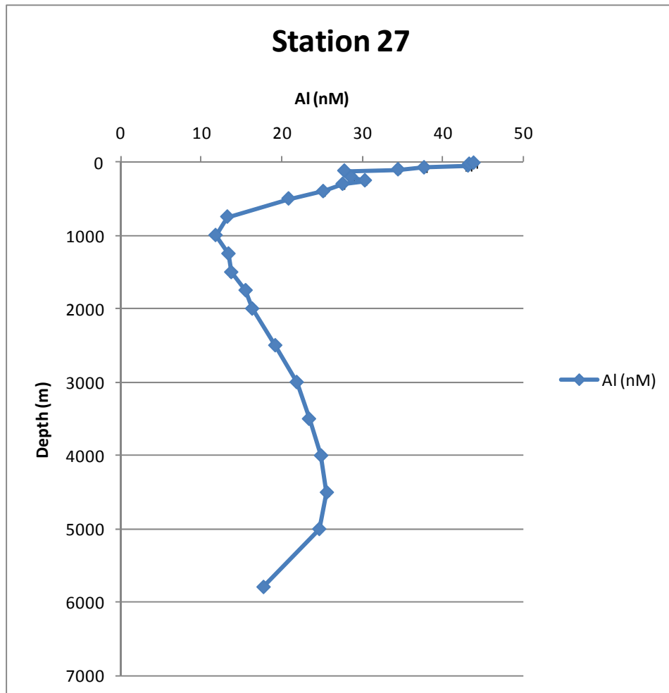
Figure 9. Dissolved Al (nM) versus depth (m) at station 27. Error bars represent standard deviation of triplicate measurement ( \sim 1\% ).
