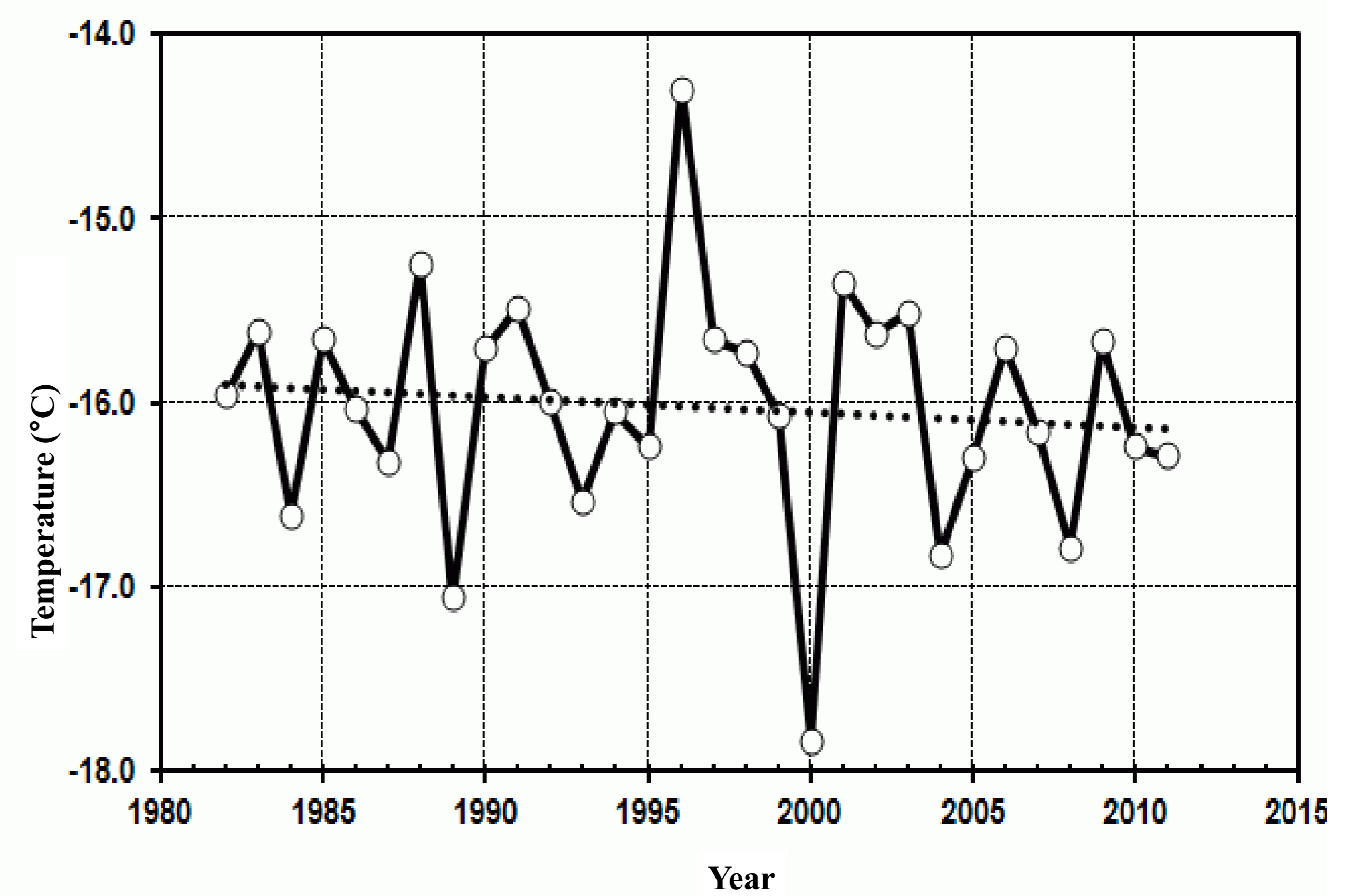
Timeseries of annual averaged air temperature
