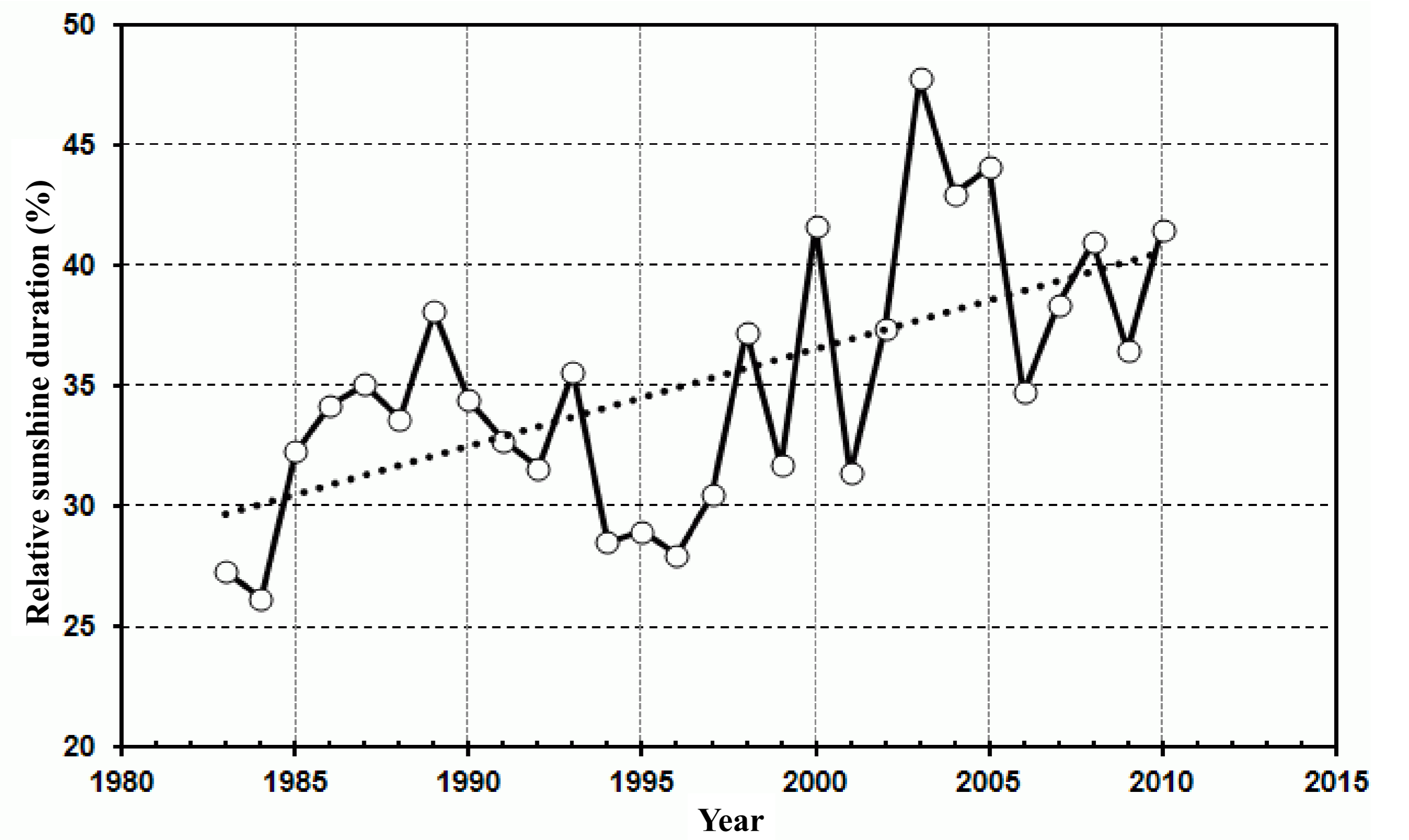
Timeseries of annual averaged relative sunshine duration
