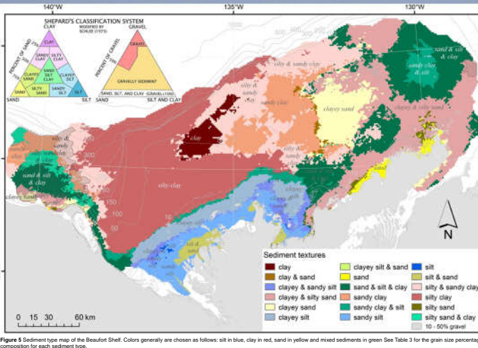
Figure 5 Sediment type map of the Beaufort Shelf. Colors generally are chosen as follows: silt in blue, clay in red, sand in yellow and mixed sediments in green. See Table 3 for the grain size percentage composition for each sediment type.
