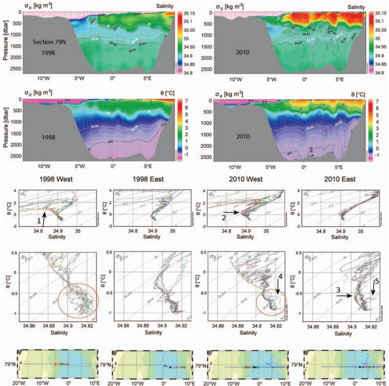
Figure 3. (Upper panels) Salinity (upper) and potential temperature (lower) sections along 79°N in 1998 (left) and 2010 (right). The lower part shows \theta - S curves from the western and eastern parts of the strait, upper diagrams being full scale and lower diagrams blow-ups of the deeper layers, 1998 to the left, 2010 to the right. The positions of the stations are indicated by coloured dots on the maps of the sections at the bottom. (1) Cold AAW from the Canadian Basin seen in 1998. (2) The less-saline salinity minimum present in 2010, perhaps the result of it incorporating the cold, less-saline AAW core. (3) The AIW salinity minimum in 2010, which is not as distinct in 1998, circles indicating the part of the \theta - S space between the Arctic Ocean and NDWs that is occupied by interleaving, which was much stronger in 1998 than in 2010. (4) The sole distinct CBDW present over the Greenland slope in 2010. (5) CBDW characteristics present in an eddy in the eastern part of the strait.
