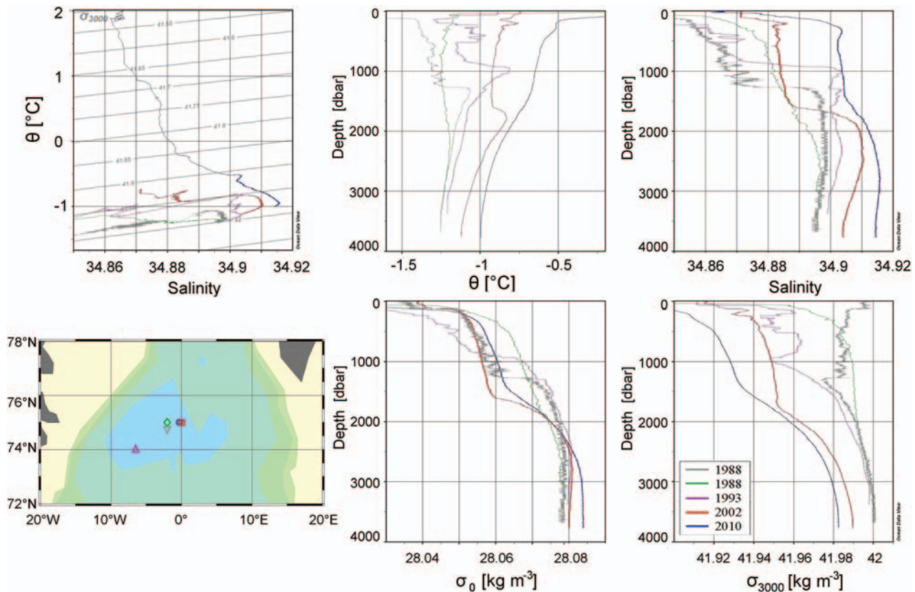
Figure 7. Profiles of potential temperature, salinity, potential density, and \sigma_3 , and \theta - S curves from two stations taken in 1988 (one in winter, grey, and one in early summer, green), one station taken in early spring in 1993 (magenta), one in early spring 2002 (red), and one in summer 2010 (blue) in the central Greenland Sea. The 1988 stations show almost active convection in winter and subsequent overturning before summer. Because of the low salinity surface layer present on the winter station, the convection was haline rather than thermal, which is also indicated by the more-stratified final water column. The other stations show the reformation of the deep salinity maximum and the formation, initial deepening, and final disappearance of the intermediate temperature maximum attributable to the warming of the upper layers. The salinity maximum (and the temperature maximum) increases in salinity, and the salinity maximum is displaced slightly downwards. The potential density has increased in the deepest layer, whereas the \sigma_3 has decreased. This indicates that the sea level in the central Greenland Sea should have risen during the past 10 years.
