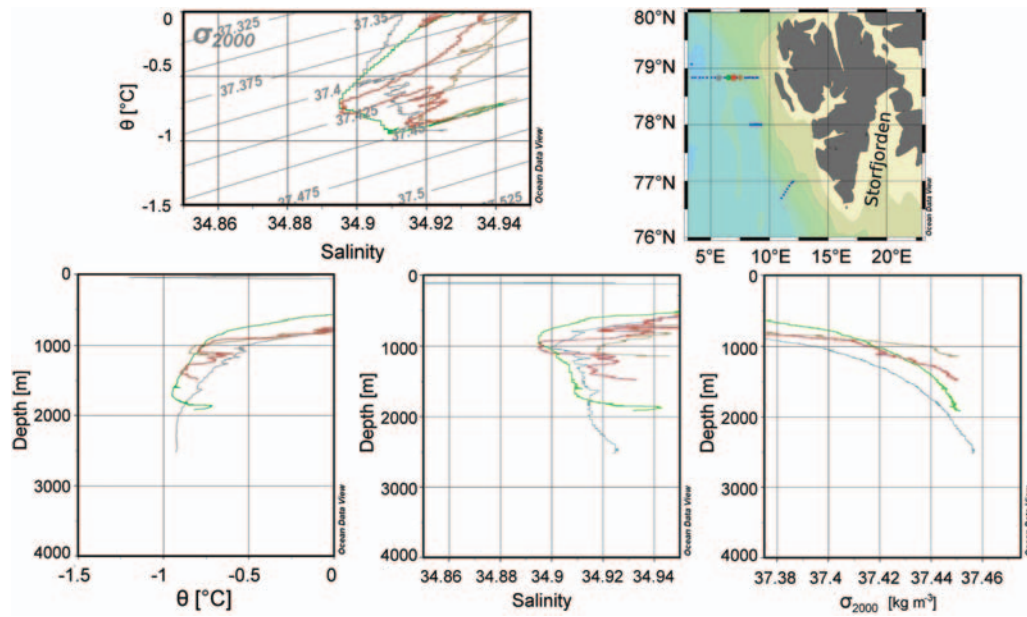
Figure 4. \theta – S curves and salinity, potential temperature, and \sigma_2 profiles from RV “Polarstern” 2002 stations taken on the 79°N section on the Svalbard continental slope, showing the sinking of a saline, dense boundary plume originating in the Storjorden outflow.
