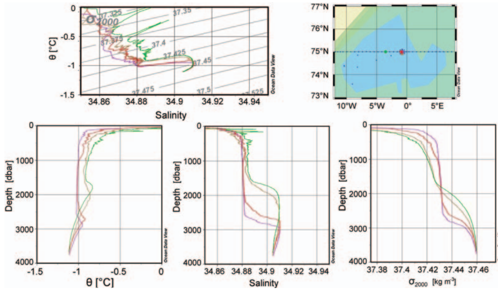
Figure 6. \theta - S curves and profiles of salinity, potential temperature, and \sigma_2 from one of the deep homogenous vortices (red and magenta stations) and from the ambient water column (green and yellow stations) observed by RV “Polarstern” in 2002. The vortex is colder, less saline, and denser in its upper part, but less dense in its lower part than the surrounding water masses, indicating that it is forced downwards dynamically, not by buoyancy. The open-ocean deep convection brings cold, less-saline water into the deep, whereas the boundary convection supplies warmer, more-saline deep water to the deeper layers (Figure 4).
