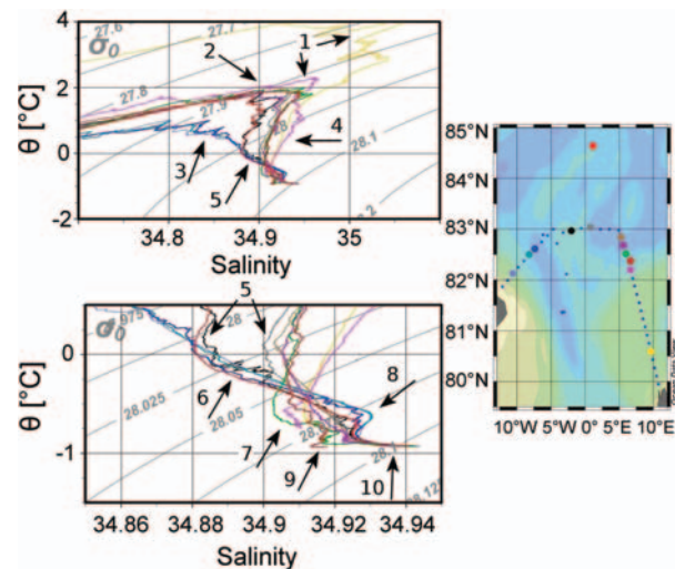
Figure 2. \theta - S curves from stations taken north of Fram Strait by RV Polarstern in 2004. The upper panel shows the full scale, and the lower panel is a blow-up of the deeper layers. Station positions are indicated by coloured dots on the map. (1) AW from the West Spitsbergen Current entering the Arctic Ocean north of Svalbard (yellow) and north of the Yermak Plateau (magenta). (2) Cooled, freshened AAW recirculating in the Eurasian Basin. (3) Colder AAW that has made the loop into the Canada Basin. (4) Denser AW entering through Fram Strait. (5) Intermediate water, uPDW in the Nansen and Amundsen basins, showing the input of less-saline Barents Sea branch water. (6) The uPDW from the Canadian Basin, where the straight \theta - S curves indicates shelf-slope convection. (7) Less-saline, colder AIW from the Greenland Sea. (8) Saline CBDW north of Fram Strait. (9) Colder, less-saline NDW entering through Fram Strait. (10) More-saline EBDW. For a more detailed water-mass classification, see Rudels (2009). Figures 2–7 have been created using Ocean Data View (Schlitzer, 2012).
