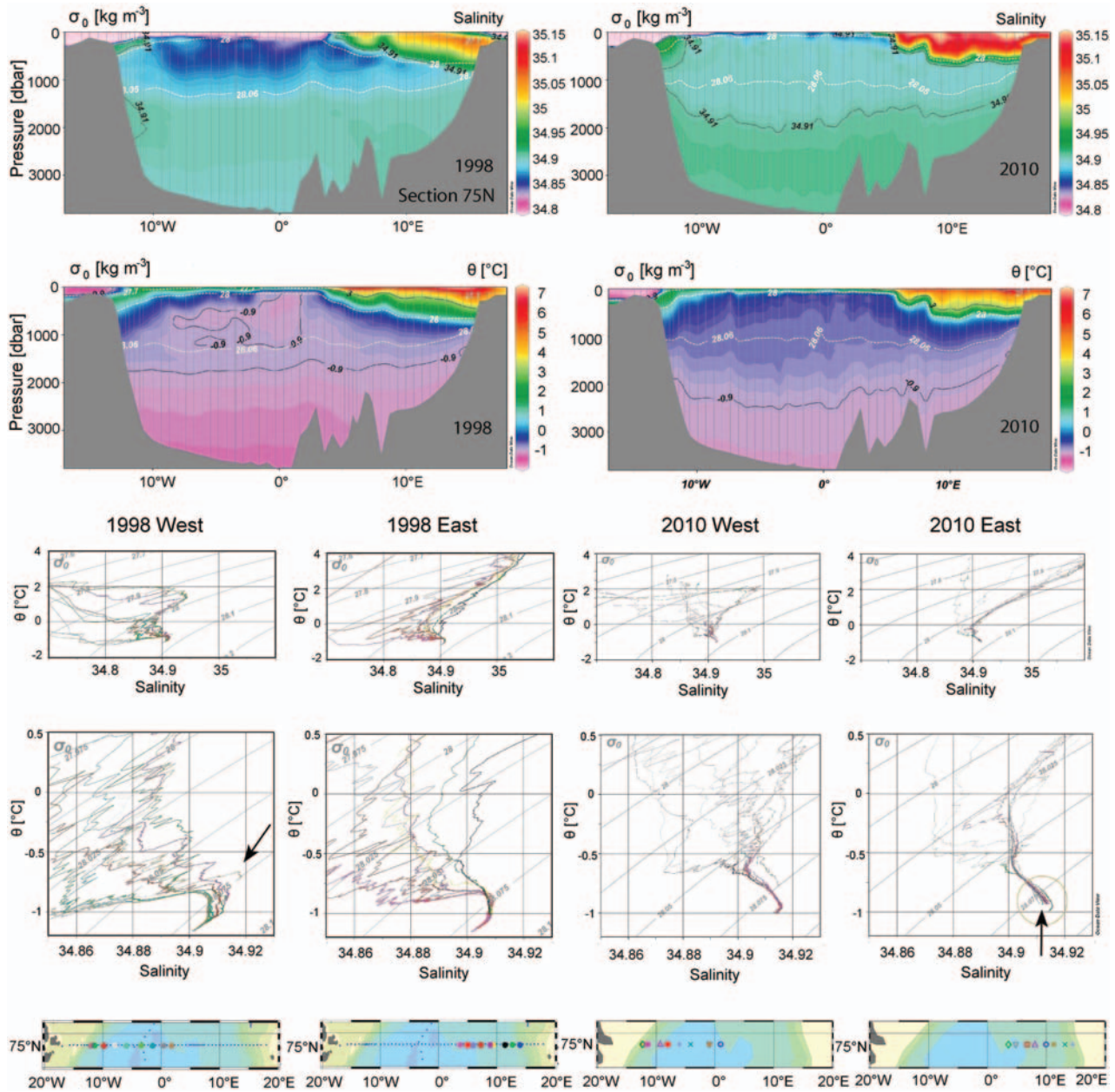
Figure 5. (Upper panels) Salinity (upper) and potential temperature (lower) sections along 75°N in 1998 (left) and 2010 (right). The lower part shows \theta - S curves from the western and eastern parts of the section, upper diagrams being full scale and lower diagrams blow-ups of the deeper layers, 1998 to the left, 2010 to the right. The arrow in the western blow-up diagram indicates the increasing salinity of the salinity maximum towards the rim in 1998, and the circle and arrow in the eastern blow-up in 2010 highlights the difference between GSDW and Norwegian Sea deep water, which has not yet been affected by saline Arctic Ocean deep waters circulating along the Mohn Ridge around the rim of the Greenland Sea.
