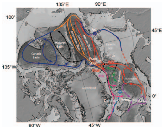
Figure 1. Map of the Arctic Mediterranean showing the sections along 75 and 79°N (broken lines) and circulation of Atlantic and intermediate water, the two inflow branches to the Arctic Ocean, over the Barents Sea (dark blue) entering at the St Anna Canyon (SAC) and the West Spitsbergen Current (WSC) entering through Fram Strait (red). The mixing between the branches along the Siberian continental slope is indicated by jagged lines, and the circulation loops in the different basins of the Arctic Ocean are shown, warm colours (reds) indicating the circulation in the Eurasian Basin and cold colours (blues) the cooler AW in the Canadian Basin. All loops join in the East Greenland Current (EGC), which in Fram Strait is augmented by the RAW. Green arrows indicate dense-water formation in and the contribution of intermediate and deep waters from the Greenland Sea. YP is the Yermak Plateau, the Eurasian Basin consists of the Nansen and Amundsen basins, and the Canadian Basin includes the Makarov and Canada basins. The circulation scheme is adapted from Rudels et al. (1994) and the map is adapted from Rudels (2009).
