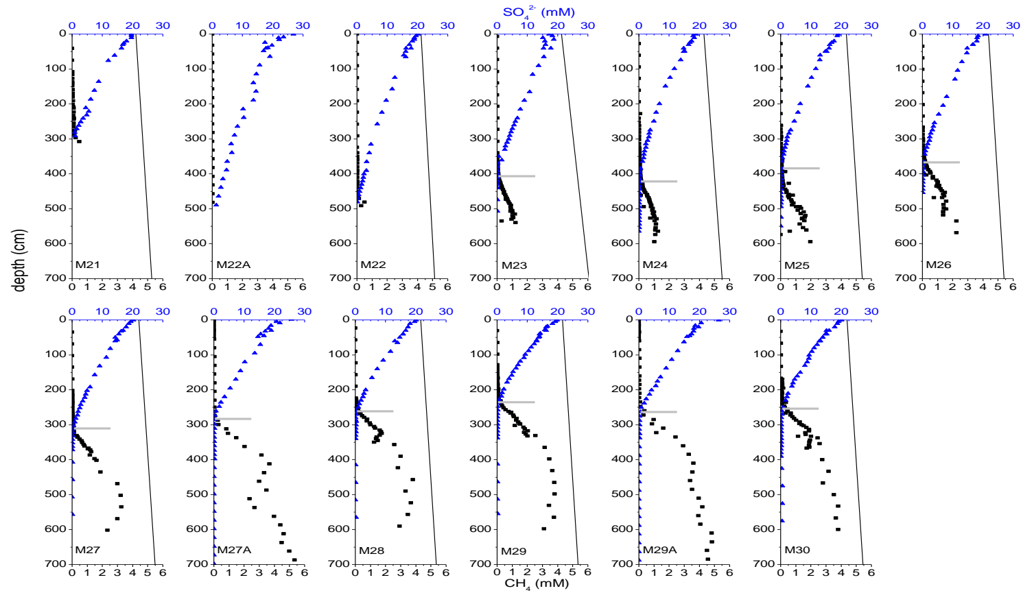
CH 4 and SO 4 2- profiles along the transect. M21-M26 are in the gas-free area with M26 ca. 12 m from the transition and M27-M30 are in the gassy sediment area. The gray line represents the peak of the SMT (defined as [CH 4 ]=[SO 4 2- ]), the fine solid black line is in situ CH 4 saturation.
