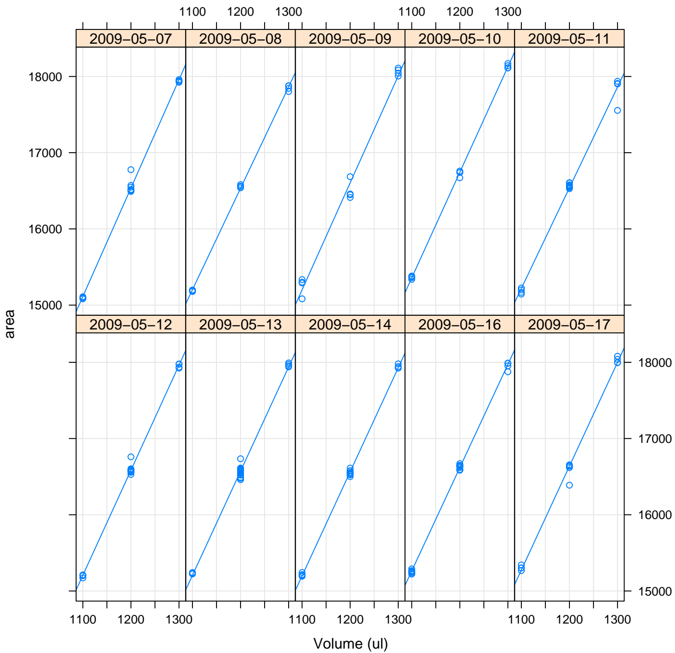
Figure 1: Regression line of area versus time with CRM 95 (13 May 2009).
