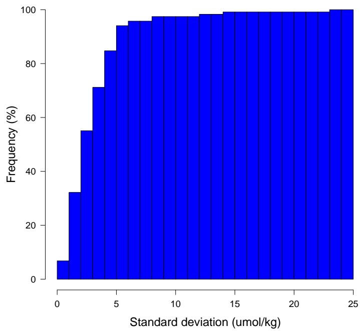
Figure 2: Cumulative frequency distribution of the standard deviation of all DIC measurements carried out during the campaign.
