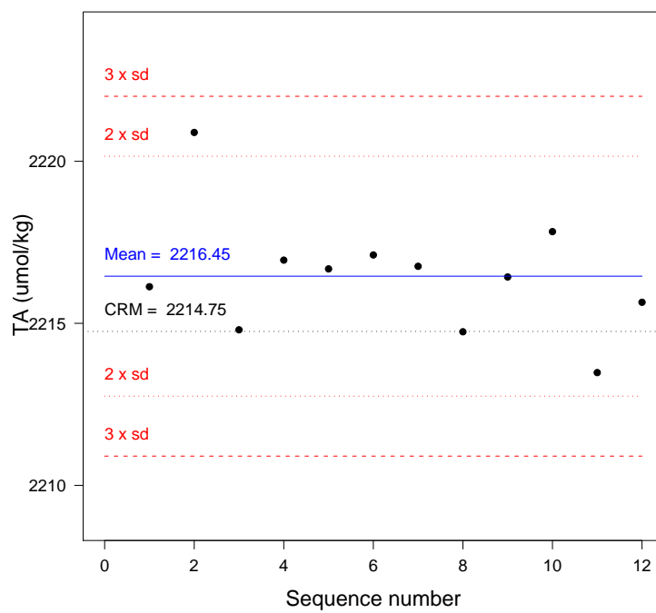
Figure 6: TA property control chart. 12 samples were measured on batch 95.
