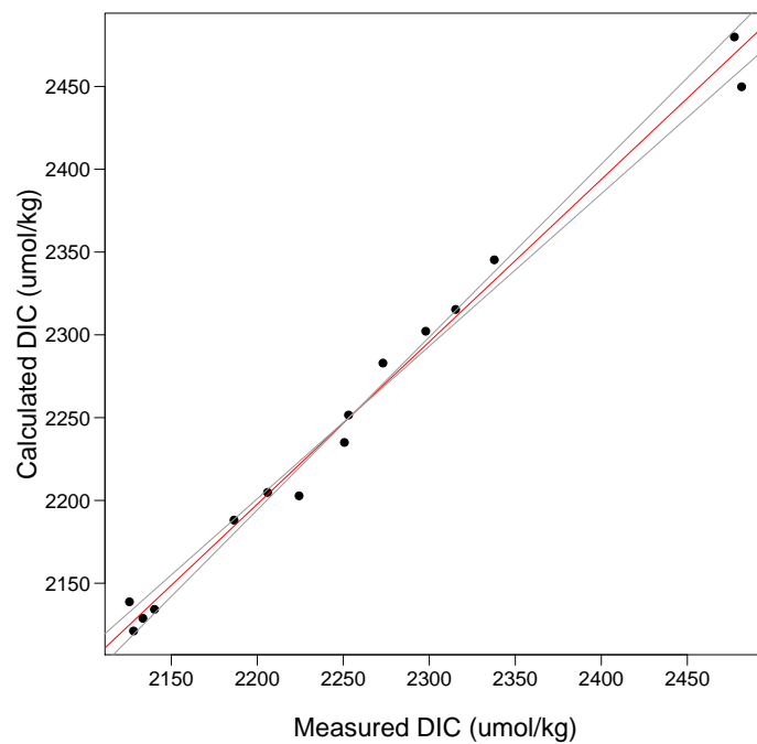
Figure 5: DIC estimated from pH and total alkalinity as a function of DIC measured with the AIRICA. Major axis model II regression [3] was used. The equation is given in the text.
