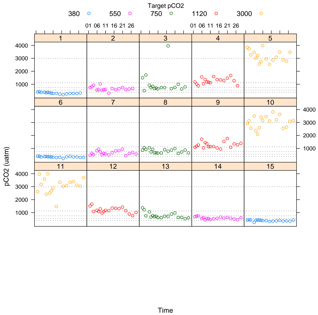
Figure 7: pCO 2 in the header tanks estimated from pH and total alkalinity measurements.
