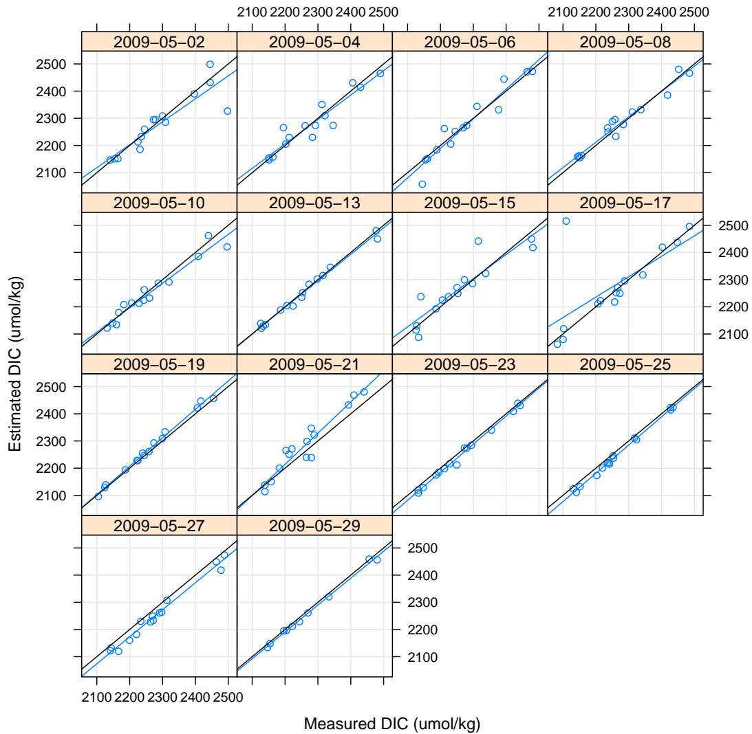
Figure 4: DIC estimated from pH and total alkalinity as a function of DIC measured with the AIRICA. The model I regression lines are shown in blue while the 1:1 line is shown in black. Note that model I regression should not be used when both variables are subject to measurement error. See text and figure 5 for the major axis model II regression on 13 May.
