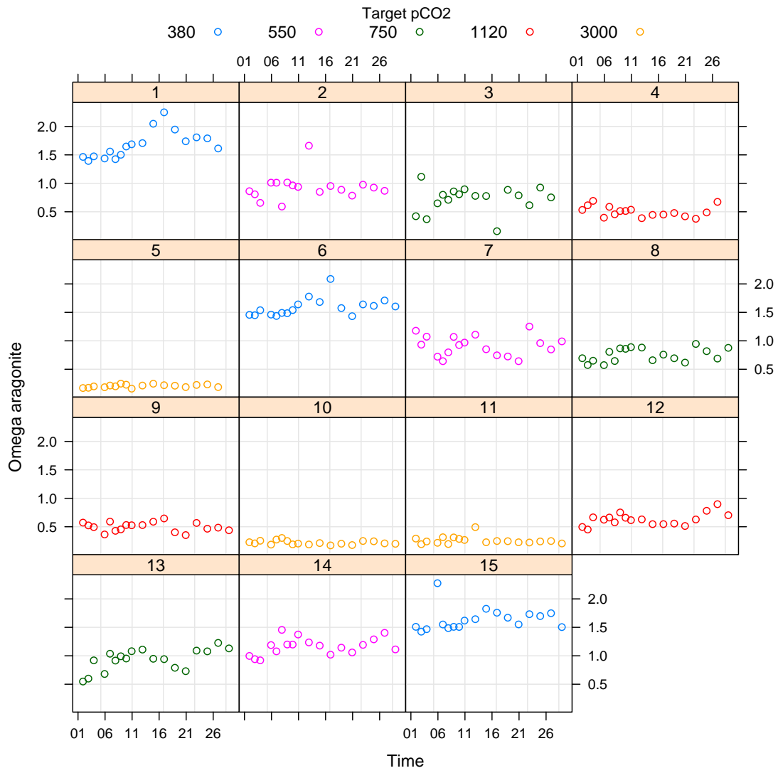
Figure 8: \Omega_{aragonite} in the header tanks estimated from pH and total alkalinity measurements.
