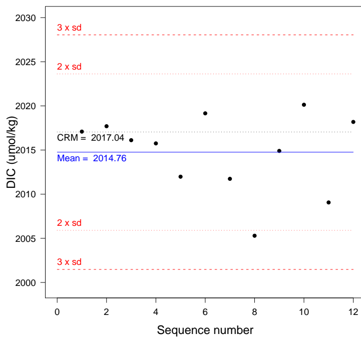
Figure 3: DIC property control chart. 12 samples were measured on batch 95. The calibration was carried out using the first 4 measurements and applied to all 12 measurements.
