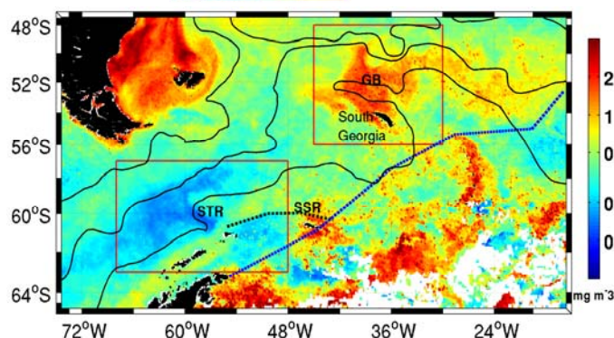
Chl-a December climatology (1997-2009); in the region south of the blue line the climatology is based on less than 6 years of data (out of 13). Data gaps due to clouds and/or sea-ice are shown in white. Red boxes indicate the two study areas surrounding the Shackleton Transverse Ridge (STR), and the Georgia Basin (GB). Fronts are from Orsi et al., DSRI 1995.
