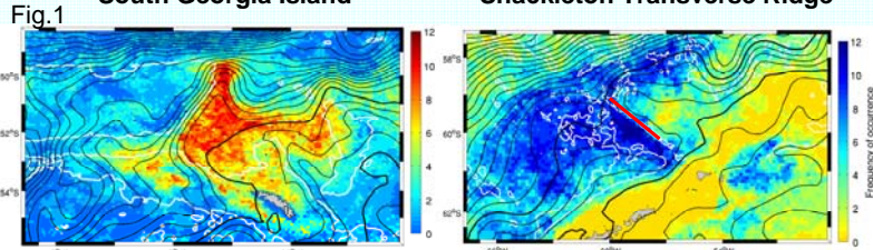
Fig.1: a) Frequency of occurrence of the high productivity range/ bloom (chl-a > 1 mg/m 3 ) around South Georgia and b) frequency of occurrence of the very low productivity range (Chla < 0.2 mg/m 3 ) around the STR. In both cases, ADT contours are overlaid (contour interval is 5cm). Values decrease from North to South and the -110cm and -90cm isolines are indicated with thick lines.
