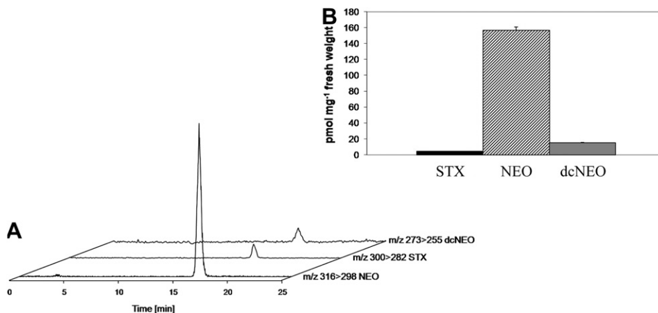
Fig. 4. LC-MS/MS analysis of PSP toxin content in C. raciborskii T3. (A) LC-MS/MS spectrum of PSP toxin components of a cellular extract. (B) Toxin content (pmol mg -1 of fresh weight).
