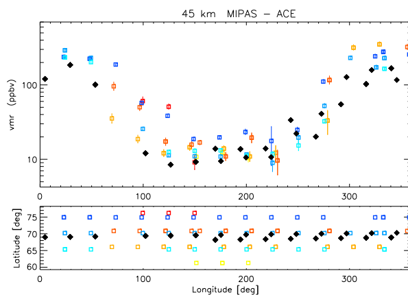
Fig. 32. Longitudinal distributions of ACE-FTS and MIPAS IMK-IAA NO x abundances measured on 18 March 2004 at VMR peak height (top) and respective geographic locations of the measurements (bottom). The error bars indicate random errors. Black diamonds: ACE-FTS, open squares: MIPAS (color coding: yellow, orange, red: daytime measurements; green, blue: nighttime measurements).
