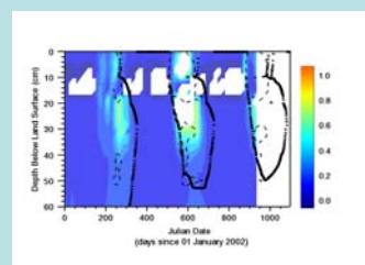
Simulation of the freeze-thaw interface (dark dots) at a hill slope site at Imnavait Creek, Alaska. The -0.1^{\circ}\text{C} isotherm (dark dashes) and unfrozen soil moisture content (background) are also shown for comparison. Color bar indicates volumetric soil moisture content. Solid white regions indicate missing data.
