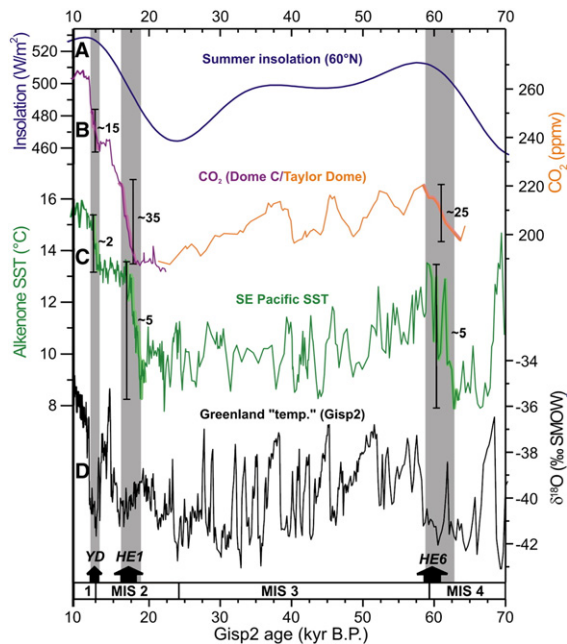
Fig. 7. Comparison of Southeast Pacific SST and atmospheric CO 2 records over T1 to the transition from MIS 4 to MIS 3. (A) Summer insolation at 60°N (Berger and Loutre, 1991). (B) CO 2 record from the Dome C (Monnin et al., 2001) (methane-synchronized to the GICC05) and Taylor Dome ice-cores (Indermühle et al., 2000). The time-scale of the Taylor Dome record has been adapted to the Gisp2-synchronized age model of the Byrd ice-core (Blunier and Brook, 2001). (C) Alkenone SST record from Site 1233 over the past 70 kyr (this study and Kaiser et al., 2005) plotted on the time-scale as published in Kaiser et al. (2005). (D) Oxygen isotope record of the Gisp2 ice-core, Greenland (Grootes et al., 1993). Intervals of substantial SST warming and CO 2 increase over T1 and at the MIS4/3 transition are marked. Numbers show approximate amplitude in ppmv and °C.
