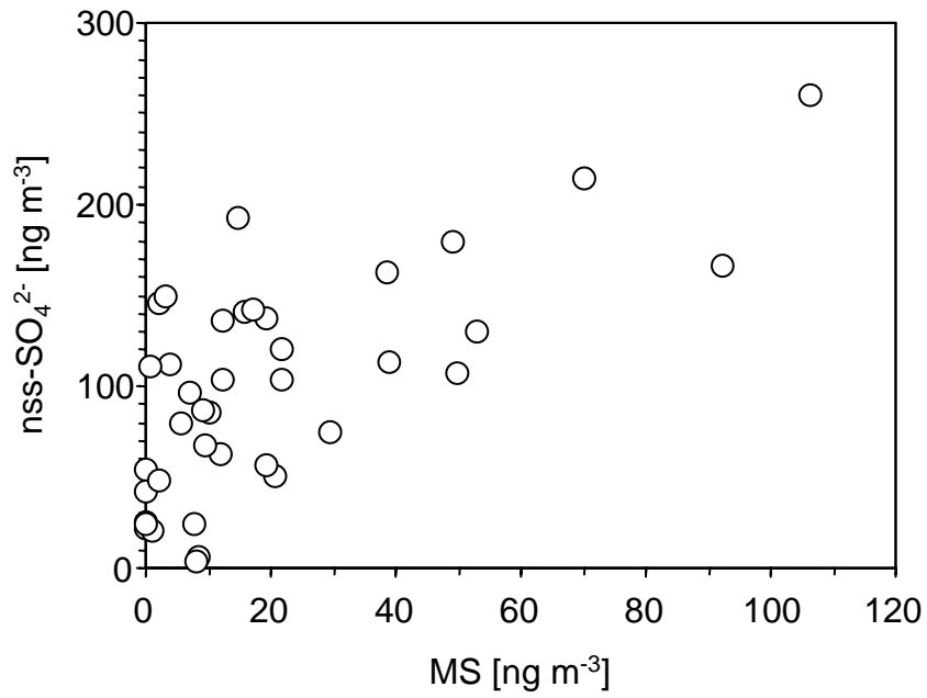
Fig. 11: Overall correlation of MS with nss-SO 4 2- concentrations (correlation coefficient r = 0.72 ).
