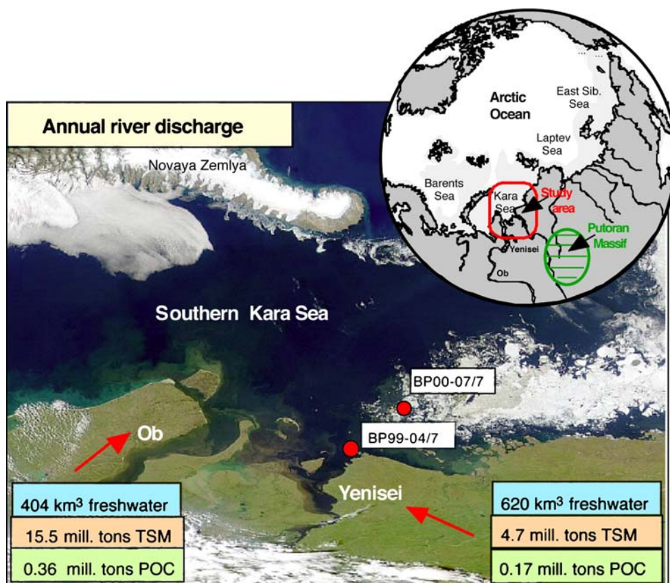
Fig. 1 Satellite photograph of the southern Kara Sea ( http://www.visibleearth.nasa.gov ), with location of cores BP99-04/07 and BP00-07/07. Values of river discharge, total suspended matter (TSM), and particulate organic carbon (POC) supply are from Rachold et al. (2004)
