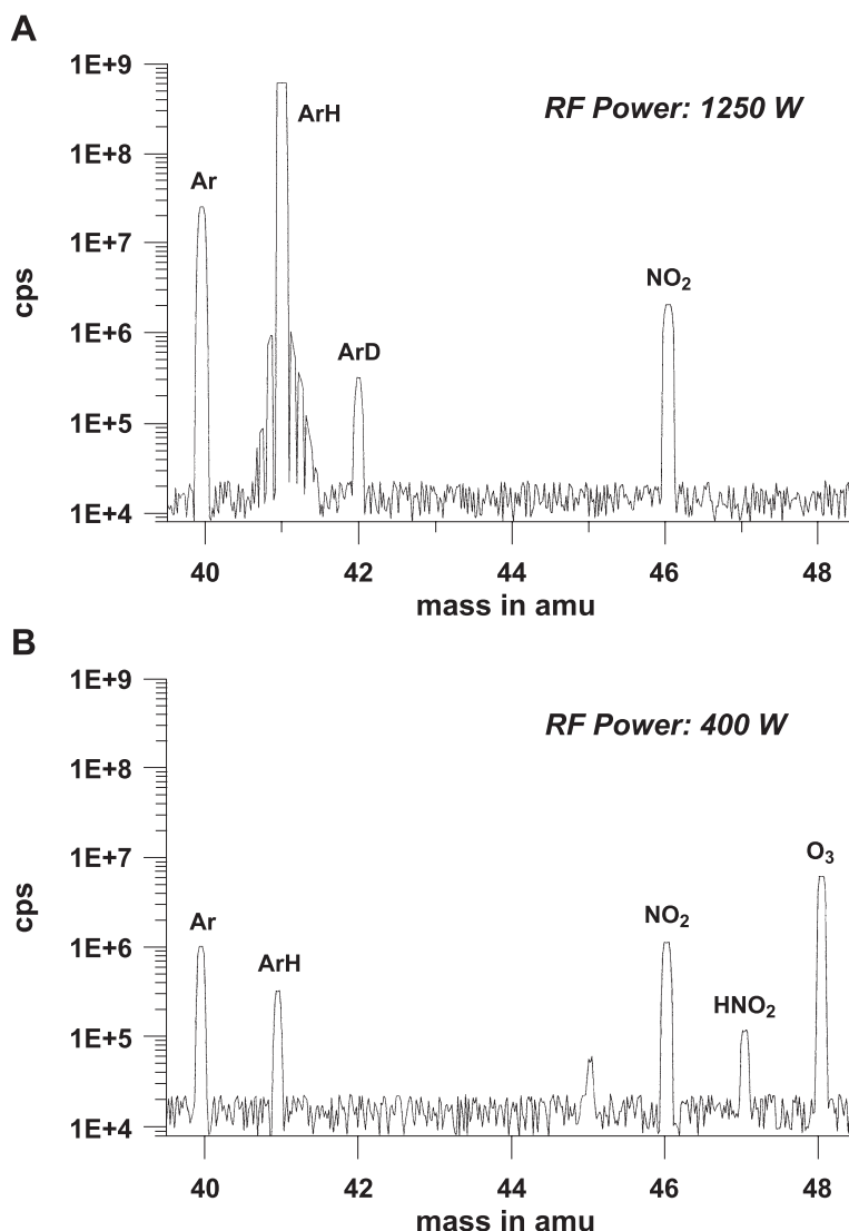
Fig. 1. The background peak intensity is shown as a function of mass in the range from 40 to 48 amu. It can be seen that the ^{40}\text{Ar}^+ intensity is significantly lower after reduction of the RF power from 1250 (A) to 400 W (B).
