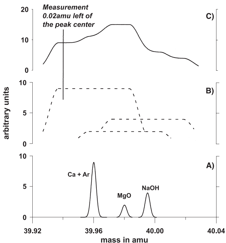
Fig. 2. Schematic drawing showing possible interfering atomic and molecular masses at 40 amu. Peak intensities are presented in arbitrary units as a function of atomic mass. (A) Using high-mass resolution (8000 Res), interfering molecular peaks can clearly be distinguished. (B) Same peaks at low-mass resolution (400 Res). (C) Integral peak plateau at 40 amu at low-mass resolution (400 Res). The mass setting used for data acquisition (0.02 towards the low-mass side of the peak center) is indicated by a vertical line. This mass setting is still on the top of the ^{40}\text{Ca} (resp. ^{40}\text{Ar} ) peak but outside the range of the interfering molecular interferences.
