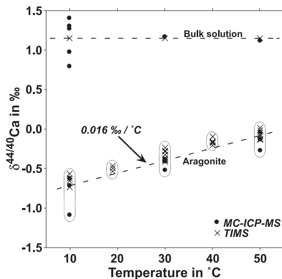
Fig. 5. MC–ICP–MS-based \delta^{44/40}\text{Ca} and TIMS-based \delta^{44/40}\text{Ca} values of inorganically precipitated \text{CaCO}_3 (aragonite; Gussone et al., 2003) are shown as a function of temperature. Within statistical uncertainties, the values of both measurements are indistinguishable from each other.
