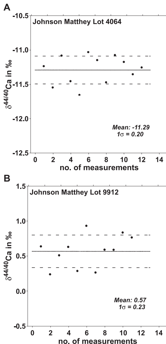
Fig. 4. MC–ICP–MS \delta^{44/40}\text{Ca} measurements of the two Johnson Matthey \text{CaCO}_3 standards, lot 4064 (A) and 9912 (B) previously used by Heuser et al. (2002) and Russell et al. (1978). The previously determined difference in \delta^{44/40}\text{Ca} of about 12 ‰ between these two standards is reproduced by the MC–ICP–MS measurements.
