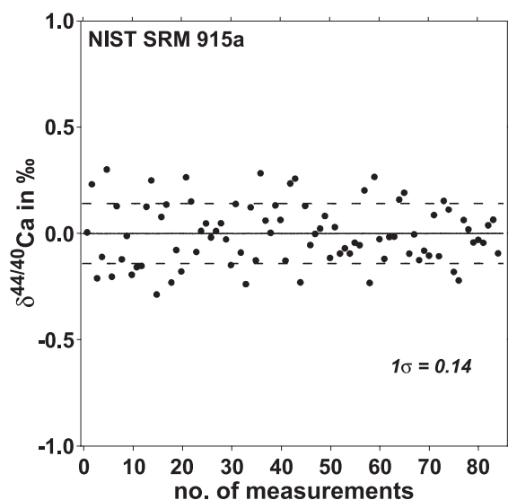
Fig. 3. MC–ICP–MS \delta^{44/40}\text{Ca} measurements of NIST SRM 915a normalized to itself. Horizontal line marks the zero mean value. Dashed lines mark the 1\sigma standard deviation of 0.14.
