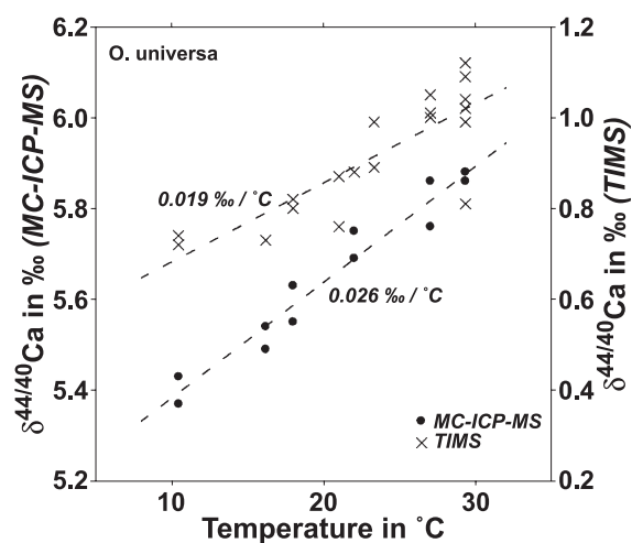
Fig. 6. MC–ICP–MS-based \delta^{44/40}\text{Ca} and TIMS-based \delta^{44/40}\text{Ca} values of O. universa samples (calcite; Gussone et al., 2003) are shown as a function of temperature. The MC–ICP–MS-based \delta^{44/40}\text{Ca} -temperature gradient is steeper than the TIMS-based \delta^{44/40}\text{Ca} gradient. Note that there is an offset between the MC–ICP–MS- and the TIMS-based \delta^{44/40}\text{Ca} values of about 5‰ caused by a matrix effect.
