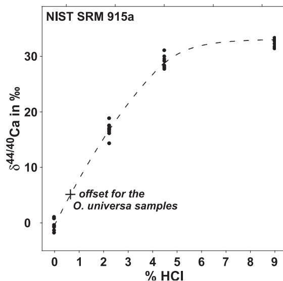
Fig. 7. This figure shows \delta^{44/40}\text{Ca} ratios as a function of HCl added to a 5% nitric acid solution of NIST SRM 915a. It can be seen that the \delta^{44/40}\text{Ca} values increase as a function of the amount of HCl added to the standard. Then, latter function can be used to correct for the observed matrix effect in the O. universa samples.
