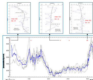
Figure 2. Snow accumulation along the Kottas Traverse in the years 1997-2001. The blue line represents a mean value for this time period. Red asterisks mark the location of snow pits, providing density profiles. Examples are shown above.
