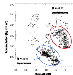
Figure 10. Envisat ASAR \sigma^0 plotted against the accumulation rate along Kottas traverse (see also Fig. 9).
