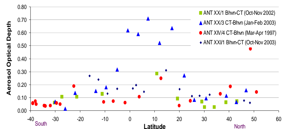
Fig. 6 Aerosol optical depth retrieved from sun-photometer data measured during four cruises of the Polarstern between Cape town and Bremerhaven. In all of these data, elevated values north of the equator indicate the presence of Saharan dust. The high AOD in the southern hemisphere are due to biomass burning aerosols coming from southern Africa.
