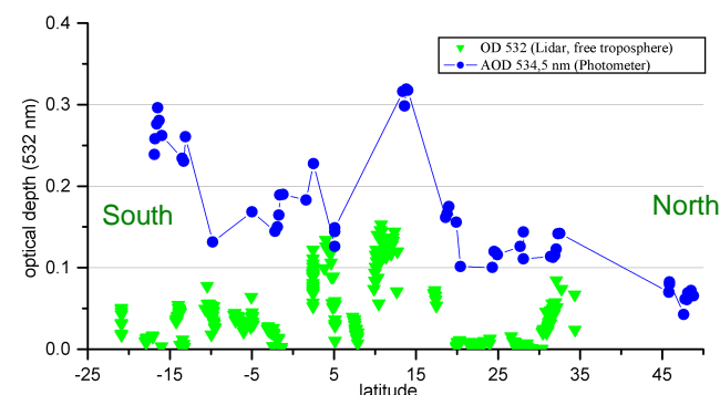
Fig. 5 Aerosol optical depth retrieved from lidar (green) and sun-photometer (blue) measurements as a function of latitude. Using the lidar data, the AOD was determined from the backscatter profiles from 0.5 to 7 km using a constant extinction to backscatter ratio of 40 sr. The green point give the AOD of the lower free troposphere (from top of PBL to 7 km).
