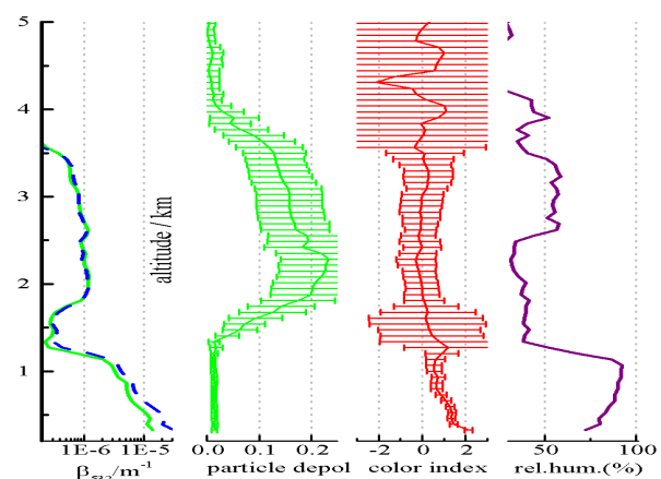
Fig. 4 Lidar profiles measured on Nov 1st, 2003 at 17°N, 20°W. Plotted is the backscatter ratio (left) particle depolarisation, the color index as the aerosol backscatter coefficient. Green: 532 nm blue 355 nm
