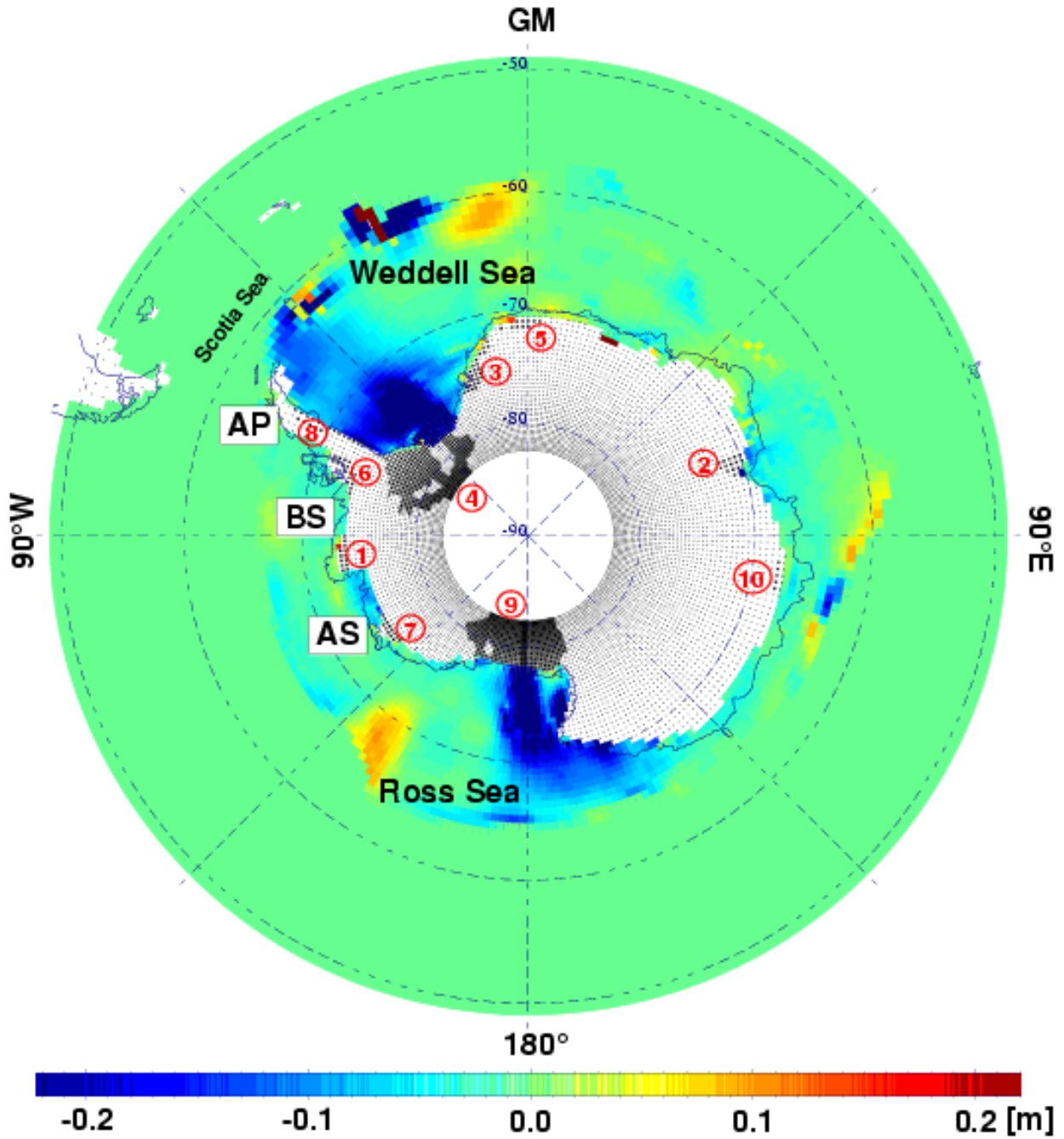
Figure 1. Difference in sea-ice thickness distribution for September of the 20 th model year in the Southern Ocean between two model configurations without ice-shelf caverns minus with ice-shelf caverns. Extreme values around South Sandwich Islands ( \sim 30^\circ\text{W} ) are due to an insufficient resolution of island passages. Circled numbers represent locations of ice shelves (dark shaded) listed in Table 1. AP: Antarctic Peninsula, BS: Bellingshausen Sea, AS: Amundsen Sea.
