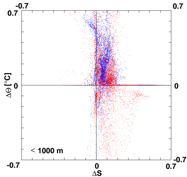
Figure 2. Annual mean (20 th model year) potential temperature vs. salinity diagram as difference ( \Delta ) between the model configurations without ice-shelf caverns minus with ice-shelf caverns separated for water column thickness less than 1000 m in the Weddell (blue) and Ross (red) Seas. Though the southern continental shelf is generally less than 500 m deep, the 1000-m threshold was chosen to include the troughs of Weddell and Ross Seas.
