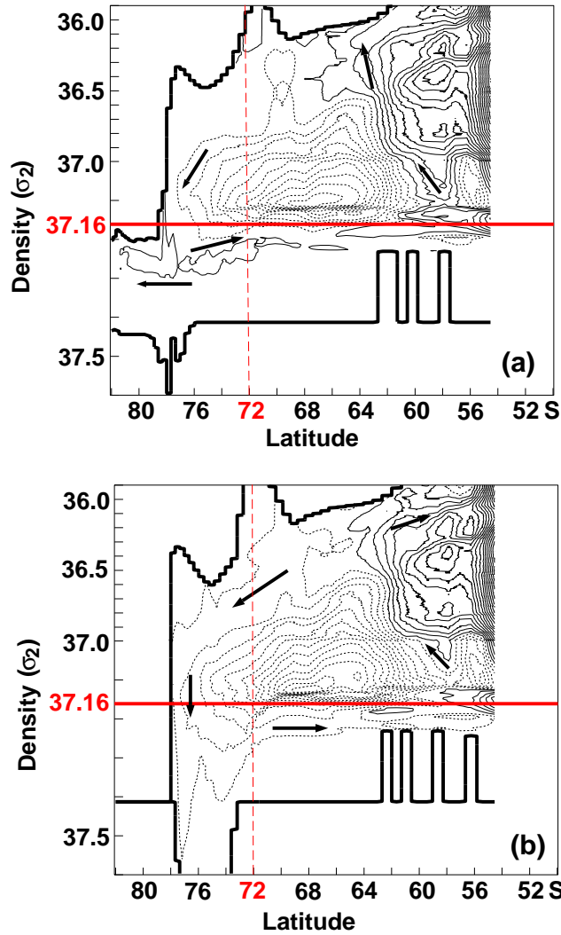
Figure 3. Annual mean (20 th model year) overturning transport streamfunction for the Southern Ocean south of 54°S for model configurations (a) with and (b) without ice-shelf caverns. For densities \sigma_2 \geq 37.0 \text{ kg m}^{-3} , the vertical scale is stretched to better present the dense water transport. Red lines mark the density \sigma_2 = 37.16 \text{ kg m}^{-3} defined as upper bound for Antarctic Bottom Water formed south of the Antarctic Circumpolar Current [Orsi et al. , 1999] (horizontal), and the approximate position of the continental shelf break in Weddell and Ross Seas (vertical). Dashed contours indicate counter-clockwise, solid contours clockwise circulations (see arrows). Bold solid lines represent the minimum (upper) and maximum (lower) density value for each latitudinal band. Contour spacing is 1 \times 10^6 \text{ m}^3 \text{ s}^{-1} starting from \pm 1 \times 10^6 \text{ m}^3 \text{ s}^{-1} .
