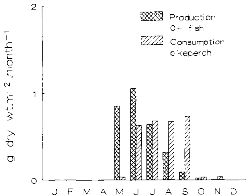
Fig. 4. Seasonal variation in the total production of O+ fish (g dry wt m -2 month -1 ) and the consumption by pikeperch (g dry wt m -2 month -1 ).
