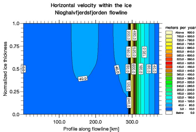
Figure 5: Horizontal velocity component in a vertical transect along the Nioghalvfjærdsfjorden flowline.
