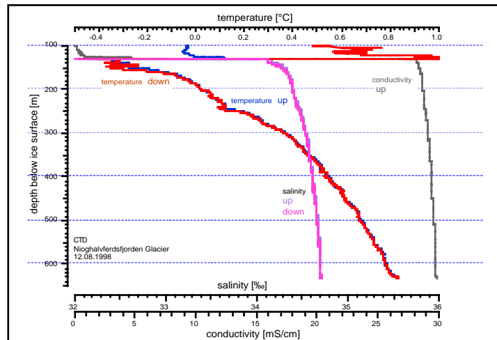
Figure 1: CTD profile obtained from a borehole at the GEUS Camp, Nioghalvfjerdingsfjorden Glacier
