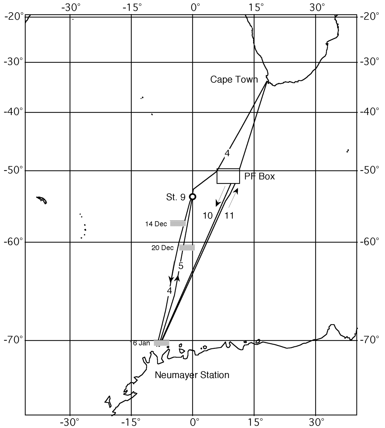
Fig. 1 Cruise track with numbers of transects as indicated in Fig. 3, the approximate position where the transects crossed the ice edge (hatched), the position of Station 9, and the intensively studied Box near the Polar Front.
