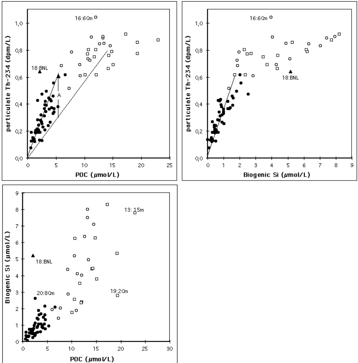
Fig. 4. Particulate ^{234}\text{Th} (dpm/L) as a function of POC (particulate organic carbon, a) and biogenic silica (BSi, b) and BSi versus POC (c) in all samples from the Polar Front area ( 49^{\circ}30' to 51^{\circ}30'S ) where BSi was measured, distinguishing samples from the surface water (open squares), from 20-60 m depth (open circles) and from below 80m (closed symbols) with regression lines through the origin (eqs. 1 and 2). One sample from the benthic nepheloid layer (BNL, triangle) at station 18 depicts the influence of resuspended surface sediments.
