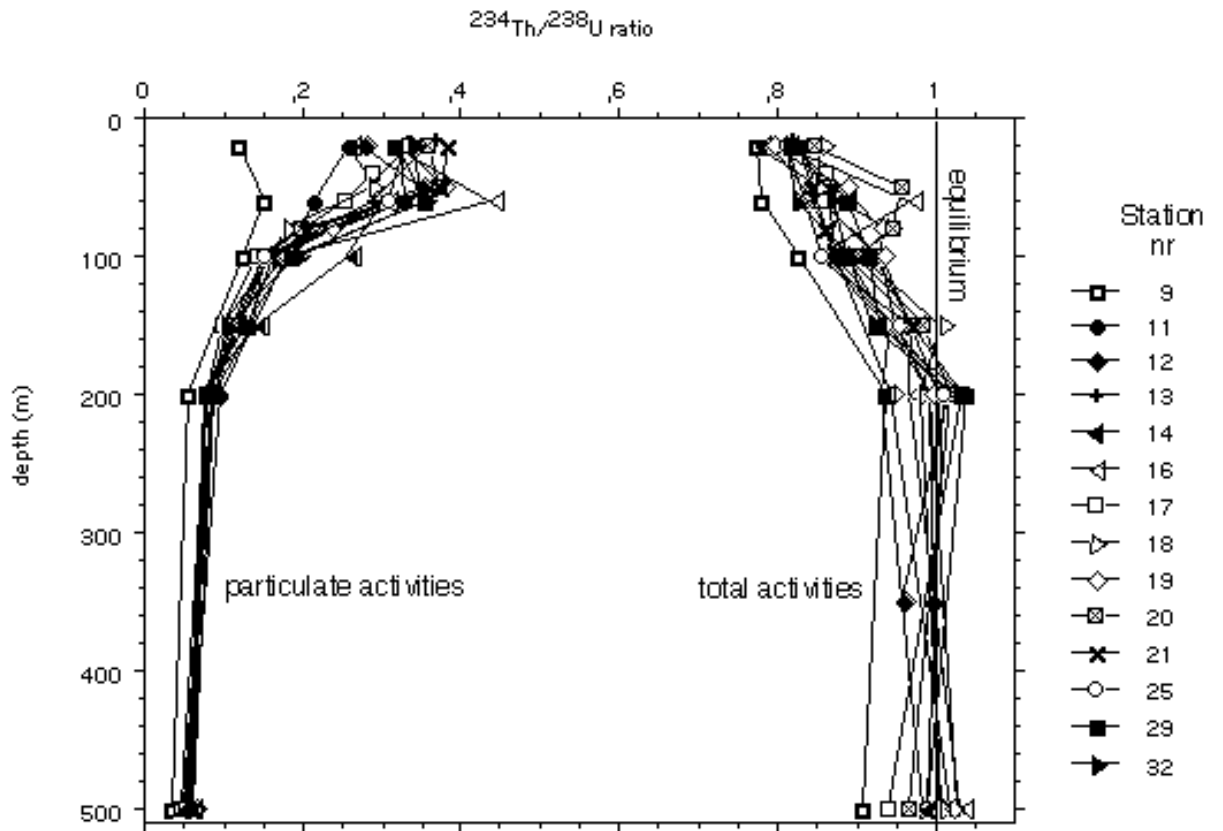
Fig. 2. Depth profiles of particulate (left) and total (right) ^{234}\text{Th} activities, presented as ratio to the activity of the parent nuclide ^{238}\text{U} (1 = secular equilibrium).
