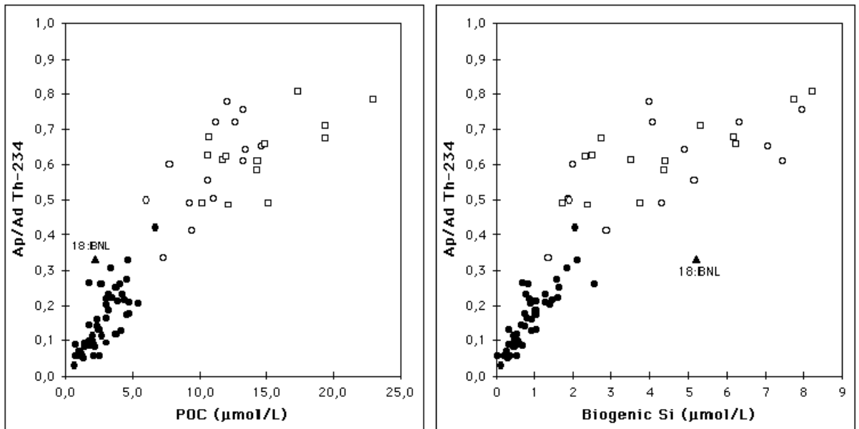
Fig. 5. The ratio of particulate to dissolved ^{234}\text{Th} activity as a function of POC (a) and BSi (b). Symbols as in Fig. 4.
