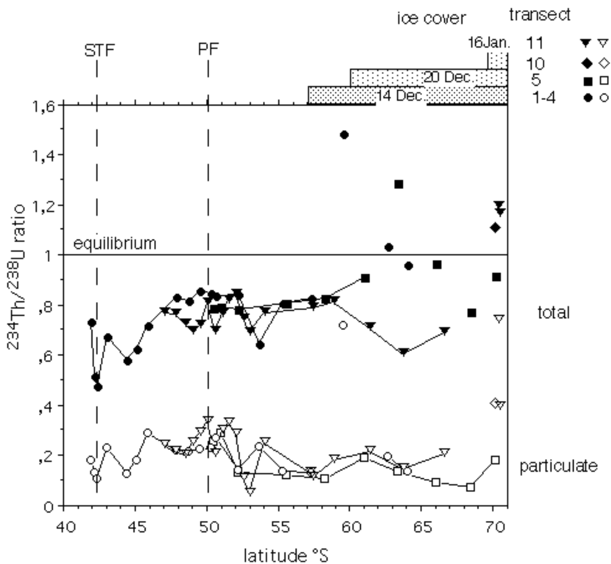
Fig. 3. Particulate (open symbols) and total (closed symbols) ^{234}\text{Th} in surface water, expressed as a ratio to ^{238}\text{U} , over the various N-S transects, showing the depletion of total ^{234}\text{Th} relative to ^{238}\text{U} near the Subtropical Front (STF), at 44:30°S and at 54°S (Station 9) compared with the moderate depletion in the Polar Front (PF) Box. The excess activities in the south are ascribed to accumulation on ice algae.
