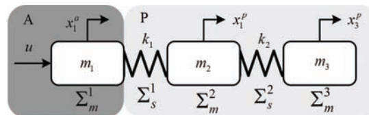
Fig. 1. Dynamical system with single input ( u ) consisting of subsystems A and P. Subsystem P has state variables which are inaccessible for measurement, whereas measurements can be taken from subsystem A. Effort-force along the power-conserving interconnection of subsystems A and P is considered as a natural feedback and utilized in the design of an energy-based state observer to estimate the states of subsystem P from the available states of subsystem A. The mass and spring energy storage elements are labeled with \sum_m and \sum_s , respectively. Positions of the first, second and third degrees-of-freedom are x_1^a , x_1^p and x_3^p , respectively. The mass energy storage elements are m_1 , m_2 and m_3 , whereas the spring energy storage elements are k_1 and k_2 .
