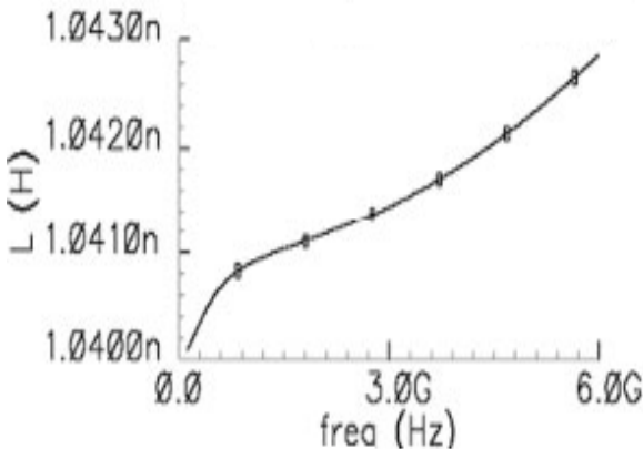
Figure 18 Inductance value of AMS library inductor.
