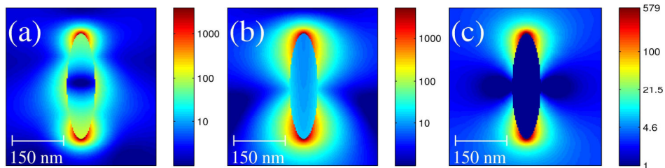
Fig. 2 Electric field intensity distribution in the vicinity of a gold prolate spheroidal nanoparticle: (a) at the quadruple resonance wavelength, (b) at the dipole resonance wavelength, and (c) at the off resonance wavelength.
