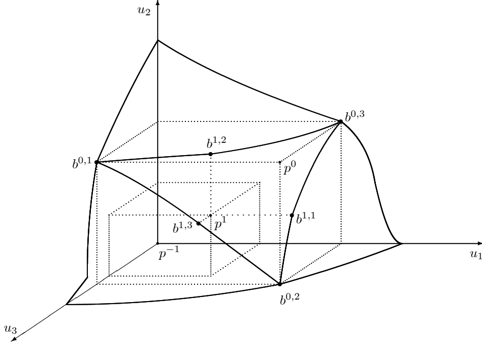
Figure 1: Constructing the brace of an arbitrary problem.
