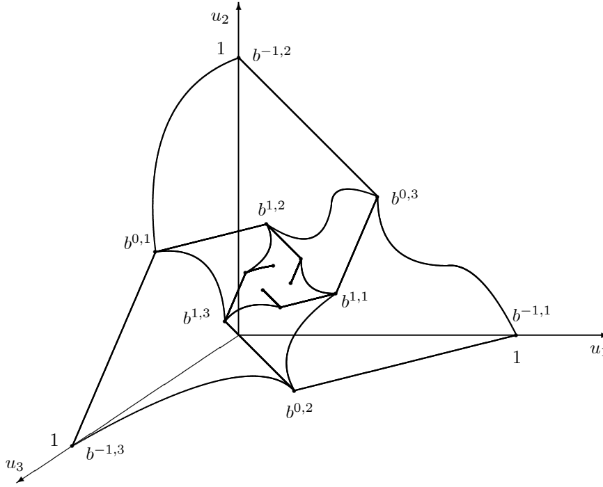
Figure 3: A typical ordinally normalized problem.
