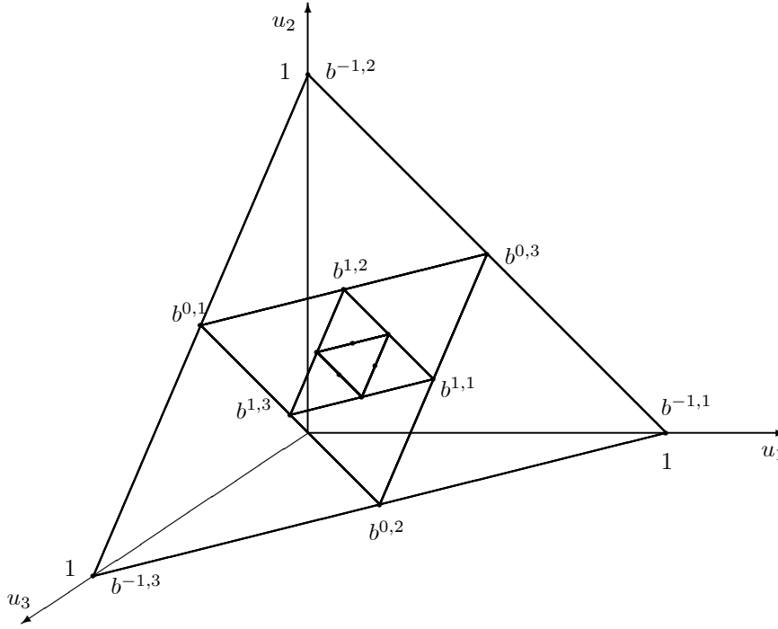
Figure 4: Constructing C^* .
