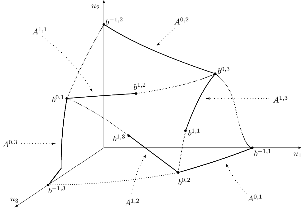
Figure 2: Constructing the extended brace of an arbitrary problem.
