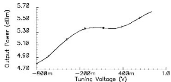
Figure 5. Fundamental frequency output power vs. differential tuning voltage.
