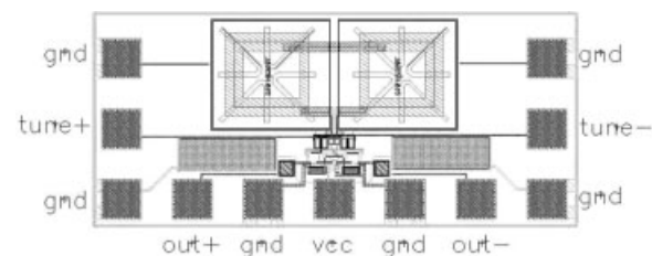
Figure 7. VCO layout.
