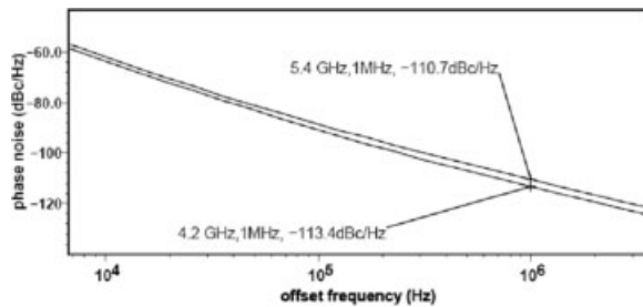
Figure 3. Phase noise of the VCO.
