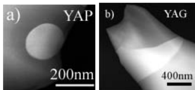
FIG. 1. ADF-STEM images of (a) YAP, and (b) YAG precipitates.
