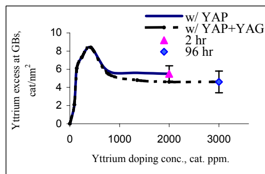
FIG. 2. Saturation \Gamma_Y with YAP and YAP+YAG
