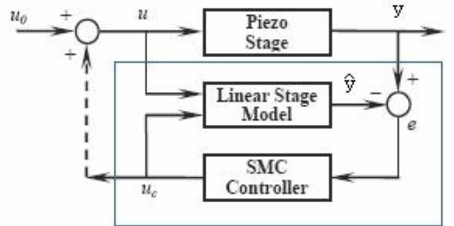
Fig.2 Observer Implementation
