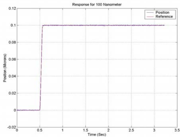
Fig. 7 Step response for 100 Nanometer
