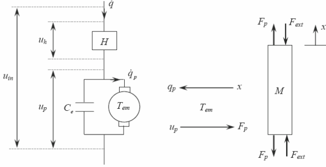
Fig. 1 Electromechanical model of a PZT actuator, [2]
