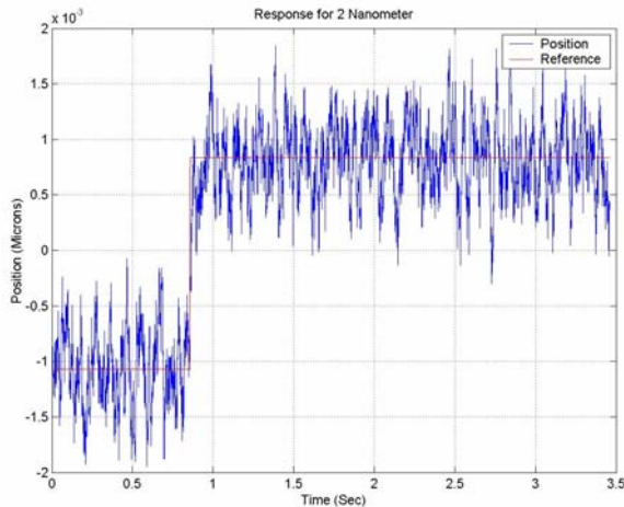
Fig. 11 Step responses for 2 Nanometer
