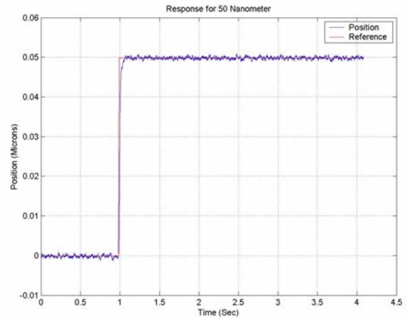
Fig. 8 Step responses for 50 Nanometer
