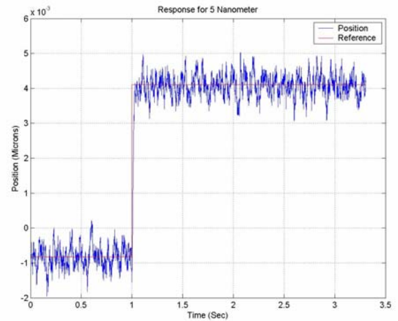
Fig. 10 Step responses for 5 Nanometer
