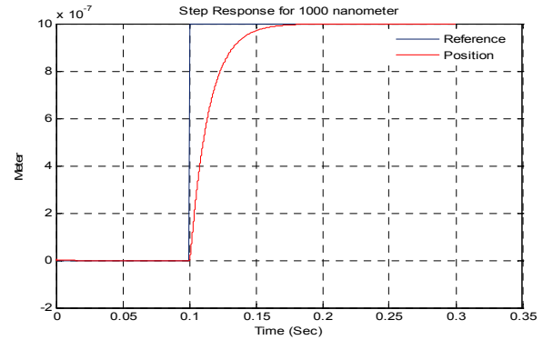
Fig. 4 Step response for 1000 Nanometer
