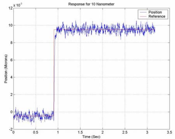
Fig. 9 Step response for 10 Nanometer
