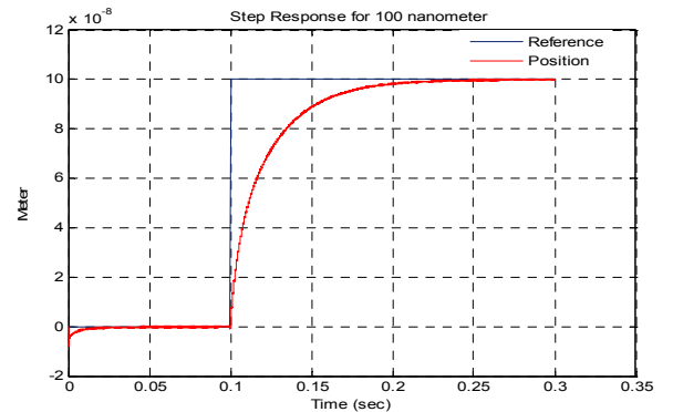
Fig. 5 Step response for 100 Nanometer
