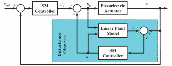
Fig. 3 Simulink Model of the overall system
