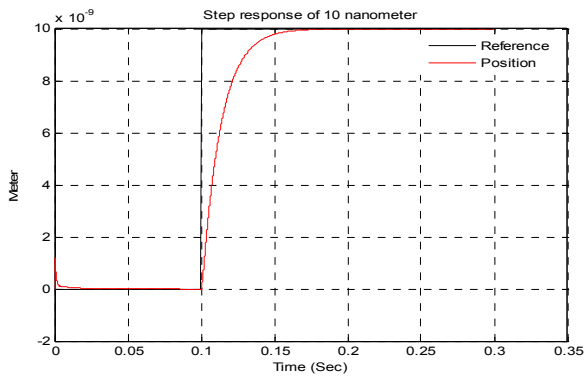
Fig. 6 Step response for 10 Nanometers
