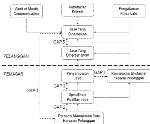
Gambar 1. Model Servqual
