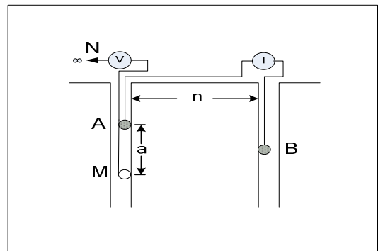
Gambar 4 Konfigurasi bipole-pole AM – B [1]
