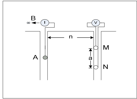
Gambar 3 Konfigurasi pole-bipole A – MN [1]
