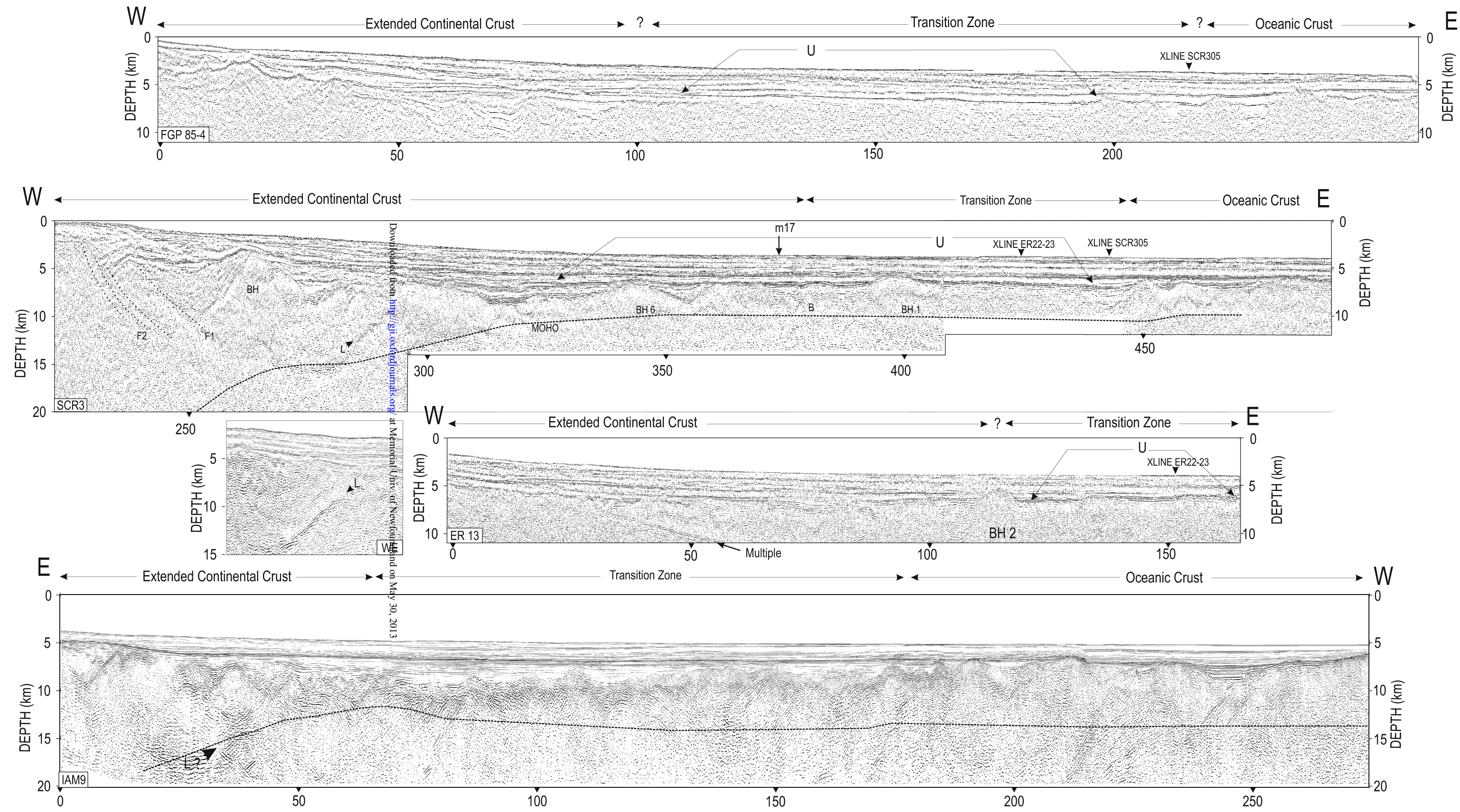
Figure 3. Seismic reflection profiles across the continental slope and rise over the Newfoundland basin and conjugate Iberia Abyssal Plain. IAM9 is plotted in reverse orientation for easier comparison with the Newfoundland Basin profiles. WE is a proprietary industry profile not located in Fig. 1 that occurs north of SCR3. SCR3 is time migrated from 170–295 km and pre-stack depth migrated from 295–470 km. FGP 85-4, ER13, WE and IAM9 are post-stack time migrated. Moho is indicated as a grey dashed line on SCR3 (from Lau et al. 2006b) and IAM9 (from Dean et al. 2000; Pickup et al. 1996). Depth conversions were made with velocity models from coincident wide-angle surveys where present (SCR3 and IAM9) and by extrapolating the SCR3 velocity model for other Newfoundland Basin profiles. F: large faults at the shelf break, BH: basement high as referred to in the text, U: widespread strong reflector found throughout the Newfoundland Basin, L: landward dipping reflection as described in the text. Vertical exaggeration 2:1.
