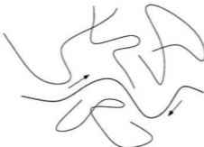
Figure 4.1: Tube model: in concentrated solutions and melts chains are restricted by neighbouring chains to motions along the contour length of the tube. The stress tensor is calculated through traction in the chains.
