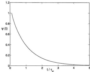
Figure 4.2: Probability distribution function in the tube, \psi(t) , as calculated by Doi and Edwards. The calculation here is for the first five terms in the sum in Eq. (4.3), for times ranging from t = \frac{1}{5} \tau_d to t = 5 \tau_d .
