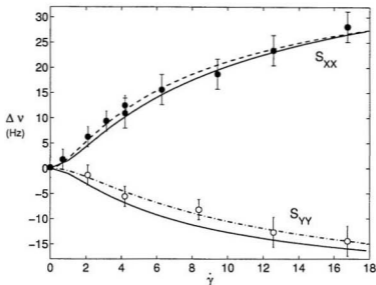
Figure 4.13: Quadrupole splittings \Delta\nu vs. shear rate for C_6D_6 in 610K PDMS melt, for Couette cell regions corresponding to velocity (solid circles) and velocity gradient (open circles) parallel with \tilde{E}_0 . The lines are fits using the Doi-Edwards model in which the absolute splitting (vertical axis) is scaled to yield the pseudo-nematic order parameter and the horizontal axis is scaled to yield the tube disengagement time \tau_d . The best compromise fit corresponds to \tau_d = 330 ms.
