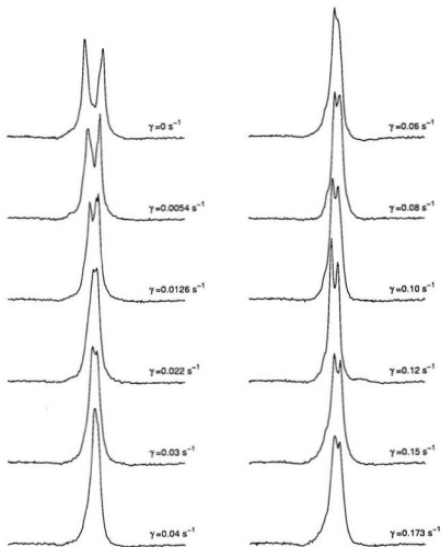
Figure 5.28: Spectra of PBLG acquired under steady shear in the 20^\circ cone and plate. Spectra were acquired at exactly 60 s following start of shear, with 2 s acquisition time in each case. The width of each spectrum is 1 kHz.
