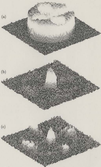
Figure 3.7: Experimentally determined spatial profiles of polymer liquid crystal in deuterated solvent, in the four-roll mill: (a) a 2 mm layer of fluid; (b) selection in two orthogonal directions to obtain signal from a 4 mm square region in the centre of the 18 mm diameter cell; (c) selection of 2.5 mm square region results in significant signal from the extra-slice wings. The images were obtained using a locally constructed 20 mm ^2\text{H} Helmholtz coil.
