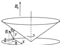
Figure 5.27: Geometry of the director reorientation in the cone and plate shear field. Velocity direction X is tangential to the rotating cone and perpendicular to the magnetic field, the velocity gradient direction Y is vertical across the gap and coincident with the magnetic field, and the third, vorticity axis is in the radial direction. The director magnitude is exaggerated and the shaded region represents the liquid crystal polymer sample. The actual angle between the cone and the plate is 20^\circ .
