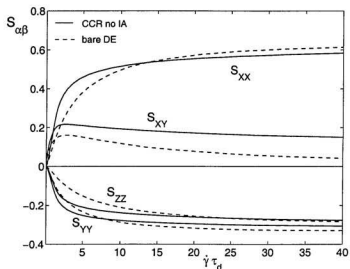
Figure 4.17: Predictions of the modified DE model (solid curves), incorporating CCR, for elements of the segmental alignment tensor S_{\alpha\beta} as a function of reduced shear rate. Dashed curves indicate predictions of the bare DE model.
