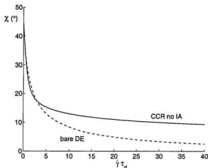
Figure 4.18: Prediction of extinction angle \chi(\dot{\gamma}\tau_d) for the modified DE model with convected constraint release (solid curve). The dashed line indicates the theoretical \chi for the bare DE model.
