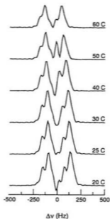
Figure 5.5: Spectra for different temperatures of PBLG at 30% concentration in dioxane- d_6 / nitrobenzene, in the quiescent state. Over this temperature range there is no observable dependence on temperature of the nematic state at rest.
