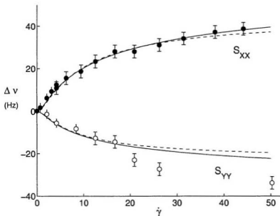
Figure 4.20: S_{XX} and S_{YY} NMR data over the full shear range. Also shown are curves for DE theory with CCR (solid line) and without (dashed line), calculated using the parameters for the fits to \dot{\gamma} < 20 \text{ s}^{-1} data and extended to \dot{\gamma} = 50 \text{ s}^{-1} .
