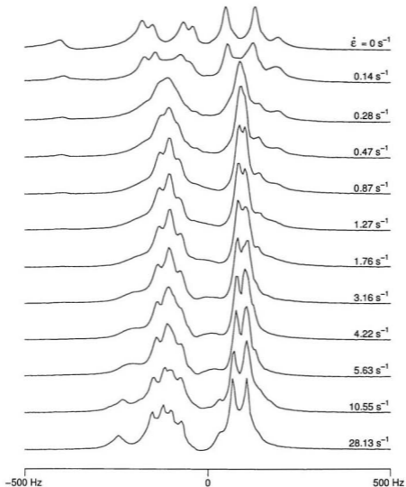
Figure 5.10: ^2\text{H} NMR spectra for PBLG at 17% concentration in the two deuterated solvents. The spectral width in the figure is 1 kHz. At this lower concentration the quadrupolar splittings in the spectra are smaller than those observed in the 20% sample. Again the splittings decrease to zero and then reappear with increasing rate of extension, as the director becomes oriented along the extension axis for \dot{\epsilon} > \dot{\epsilon}_c .
