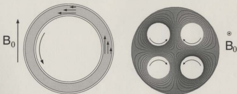
Figure 2.1: Cross-sectional views of rheometric devices. Left : horizontal Couette cell. Right : four-roll mill extensional flow cell. Shaded regions are occupied by the sample and in each case the cell is self-contained. Arrows indicate direction of mechanical driving, with fluid streamlines shown for the four-roll mill. The direction of the magnetic field, designated by B_0 , with respect to the rheometric cells is indicated in the figure.
