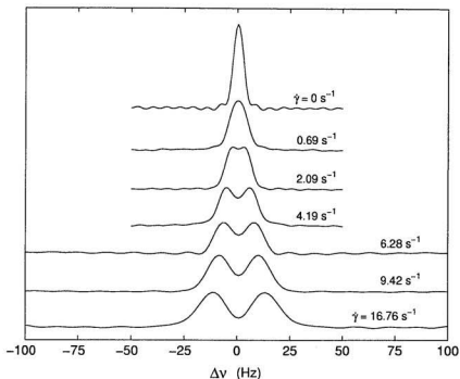
Figure 4.10: Spectra for S_{xx} , acquired using the pulse sequence described in section 3.3, at a range of shear rates for 610K PDMS melt containing the C_6D_6 probe at 10%, obtained with velocity direction parallel to the magnetic field. The width of the spectrum is determined by the evolution time t_1 in each NMR experiment.
