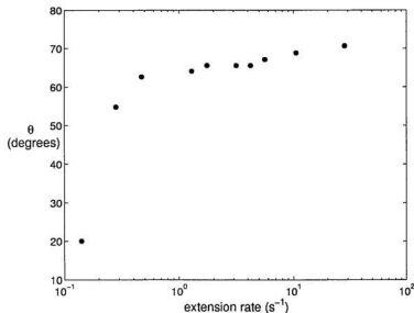
Figure 5.9: Director orientation \theta of 20% PBLG under extension in the four roll mill, plotted as a function of \dot{\mathcal{E}} . The critical extension rate \dot{\mathcal{E}}_c is estimated to be between 0.14 and 0.28 s^{-1} .
