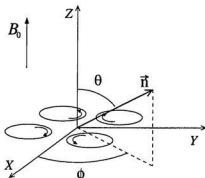
Figure 5.7: Geometry of the director reorientation in the four-roll mill extensional flow field, for extension along the x axis and compression in the y direction. The shaded region represents the nematic liquid crystal polymer solution. The (exaggerated) local director is represented in spherical polar coordinates.
