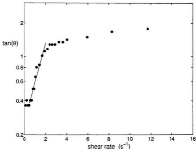
Figure 5.26: The low shear rate fit of \ln(\tan \theta) vs. \dot{\gamma} is best shown on this axis. At low shear rates the linear behaviour observed over \dot{\gamma} = 0.6 \text{ s}^{-1} to 1.7 \text{ s}^{-1} yielded 1.39 \text{ s} for the fitted slope.
