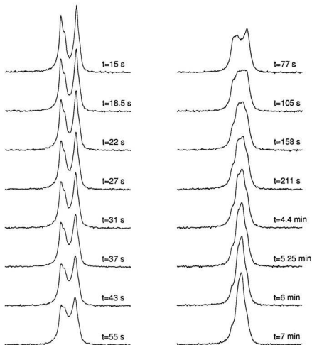
Figure 5.21: Deuterium NMR spectra of liquid crystal polymer following start of steady shear at \dot{\gamma} = 0.47 \text{ s}^{-1} in the vertical Couette cell. The spectral width is 1 kHz, with the corresponding times shown to the right of each spectrum.
