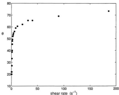
Figure 5.25: Analysis of director orientation as a function of \dot{\gamma} , in shear flow in the vertical Couette cell. The data yields two regions of orientation behaviour, which may be attributed to a change in the viscosity coefficients as the molecules become aligned with the flow, and possible development of texture.
