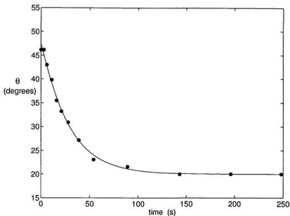
Figure 5.20: Recovery of magnetically aligned state following shear at 185.5 \text{ s}^{-1} in the vertical Couette cell. The splittings were extracted from the NMR spectra of Fig. 5.19, taking \Delta\nu_{\text{max}} = 146.5 \text{ Hz} to be the magnetically aligned orientation and \theta_0 = 20 degrees, and are plotted here as a function of time. The solid line is the fit to the predicted recovery of the magnetically aligned state in the LEP model, given by Eq. 5.8. The fit yields \chi_a B_0^2 / \mu_0 |\alpha_3 - \alpha_2| = 0.037 \text{ s}^{-1} \pm 2\% .
