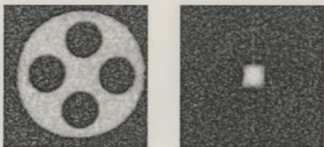
Figure 5.6: ^2\text{H} NMR images in the four roll mill, obtained on 20% PBLG solution. An image of the entire sample at left shows the four roll mill on cross-section. At right, the selection technique is used to define within the cross-section a (4\text{ mm})^2 region around the stagnation point, on which ^2\text{H} NMR spectroscopy experiments are performed.
