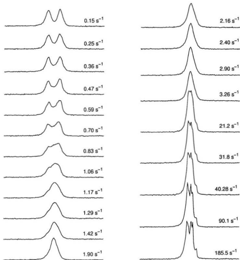
Figure 5.24: Spectra of 20% PBLG at increasing rates of shear in the vertical Couette cell. The spectral width in the displayed spectra is 1 kHz.
