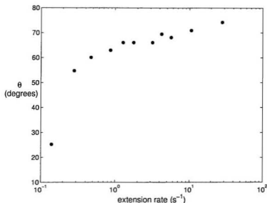
Figure 5.11: Director orientation \theta for 17% PBLG under extension in the four roll mill, plotted versus \dot{\mathcal{E}} . The data indicates a critical extension rate between 0.14 and 0.28 s^{-1} .
