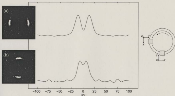
Figure 3.5: Representative ^2\text{H} NMR spectra obtained using the selective storage technique, for a deuterated benzene probe molecule in a polymer melt under shear in the horizontal Couette cell. The spectra were obtained at shear rate \dot{\gamma} = 16.8 \text{ s}^{-1} and using the spectroscopy sequence of figure 3.4. The corresponding images using the selective storage precursor were obtained with the fluid at rest. At top, signal is selectively obtained from the region of the gap where \vec{v} \parallel \vec{B}_0 , and at bottom where \nabla\vec{v} \parallel \vec{B}_0 . The orientations of the hydrodynamic frame in the selected regions, discussed in section 2.2.1, are indicated in the cartoon at right.
