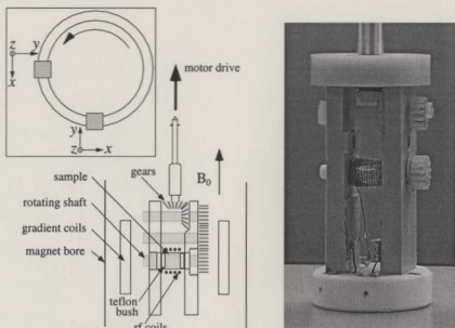
Figure 2.5: Horizontal Couette cell. The inset at left shows the hydrodynamic frame in the Couette cross-section. A photo of the assembled cell is shown at right, with one of the gears removed for the photo. The base of the apparatus fits directly onto the microimaging probe.
