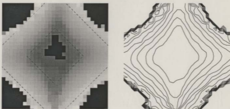
Figure 5.15: Velocity field of 20% PBLG around the stagnation point in the four roll mill, obtained via NMR velocimetry. The extension rate for this experiment is \dot{\epsilon} = 1.13 \text{ s}^{-1} . At left: speed map calculated from images acquired in two orthogonal directions in the plane of extension in the apparatus, at resolution of 0.156 \mu\text{m} per pixel. The region of interest at the centre of the four roll mill is shown here, 30 \times 30 pixels corresponding to (4.7 \text{ mm})^2 . The zero-intensity corners correspond to the rollers where no fluid is located. Highest intensity in white indicates the highest speeds near the roller edges, while very low speeds are apparent in the centre. At right: contour map calculated from the speed map, showing lines of equal velocity magnitude. The spacing of the contours reveals non-ideal features of the flow field of the liquid crystal polymer in this rheometric cell: the sharp rise in velocity gradient close to the roller surfaces, and the reduced velocity gradient in a small region around the stagnation point. The selected region for the spectroscopy experiments was oriented at 45^\circ in the plane with respect to the velocity image shown here. Dashed lines are superimposed on the image to indicate the (2 \text{ mm})^2 and (4 \text{ mm})^2 regions.
