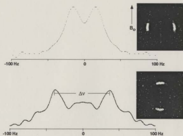
Figure 4.8: ^2\text{H} spectra for 610K PDMS melt containing the ^2\text{H} oligomer at 10% in the horizontal Couette cell at \dot{\gamma} = 12.6 \text{ s}^{-1} , obtained using the two-dimensional spectroscopy method for selected regions having velocity direction (top) and velocity gradient direction (bottom) parallel to the magnetic field. The quadrupolar splitting \Delta\nu was obtained from the doublet peaks. Corresponding images obtained using the selective storage precursor, shown to the right of each spectrum, demonstrate the selectivity of the experiment.
