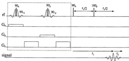
Figure 3.4: Pulse sequence showing two applications of the selective storage cluster (the portion outlined by the dashed line) followed by the two-dimensional spectroscopy experiment. The dephasing gradient shown here is applied along z , however it may equally be applied in any (or all) of the three orthogonal directions following the z -storage.
