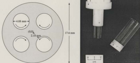
Figure 2.6: Left: dimensions of the four roll mill, drawn in cross-section, with arrows indicating direction of mechanical driving of the rollers. The distance from the stagnation point (labeled (0,0) ) to each roller edge is d = 2.18 mm. The direction of the rollers can be reversed for flow in the opposite direction. Right: photo of the unassembled cell. Each of the four rollers is 4.9 mm in diameter, and the cell holds \sim 0.5 cc. of liquid.
