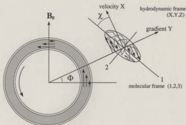
Figure 4.7: The relevant frames of reference in the horizontal Couette cell experiment.
