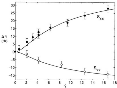
Figure 4.15: Fit of Doi-Edwards model without the independent alignment approximation to the S_{XX} and S_{YY} NMR data in the 610K PDMS melt. The fit without IA yields \tau_d = 260 ms.
