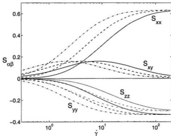
Figure 4.4: Predicted shear-rate dependence of S_{\alpha\beta} , for reptation time \tau_d = 330 ms (solid lines); \tau_d = 660 ms (dashed lines); \tau_d = 1.32 s (dot-dashed lines).
