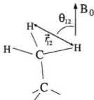
Figure 2.2: Dipole-dipole interaction between two spins whose relative positions are described by internuclear vector \vec{r}_{12} and angle \theta_{12} between \vec{r}_{12} and B_0 .
