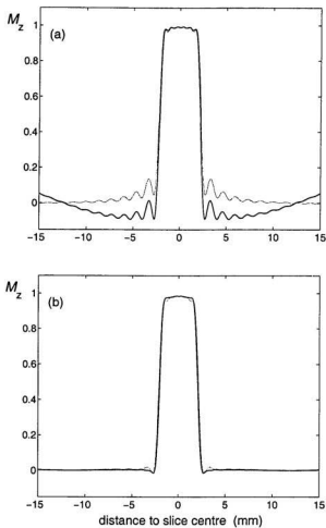
Figure 3.6: (a) Numerical results for distorted slice profile (shown in black) corresponding to application of the non-selective pulse in the presence of the magnetic field gradient. The profile is compared to that obtained with magnetic field gradient removed during the application of the broadband pulse (gray). The simulated profiles obtained for two applications of the z-storage precursor are shown in (b). T_2 = 10 ms in these calculations.
