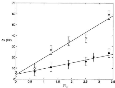
Figure 4.9: Quadrupole splittings \Delta\nu versus reduced shear rate for 610K PDMS melt containing the ^2\text{H} oligomer at 10%, obtained with velocity direction (solid circles) and velocity gradient direction (open circles) parallel to the magnetic field. Also shown is the single data point from the neutral, vorticity direction ( S_{ZZ} ) experiment (solid square). The lines drawn through the data indicate that S_{YY} increases with De roughly twice as fast as S_{XX} , which is opposite to the result expected. The S_{ZZ} data point is consistent with the velocity direction data.
