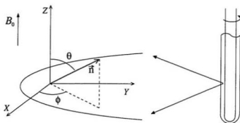
Figure 5.18: Geometry of the director reorientation in the vertical Couette shear field. Velocity X is tangential to the rotating inner cylinder, the velocity gradient Y is radial across the gap, and the third, vorticity axis is in the magnetic field direction. As in figure 5.7, the shaded region represents the sample in the Couette gap.
