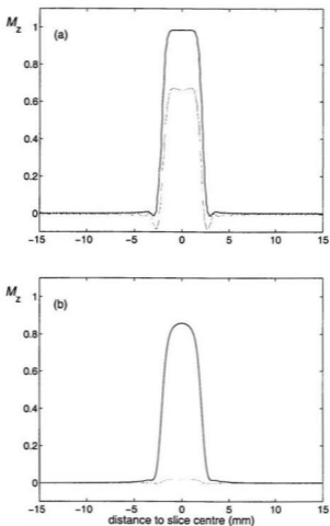
Figure 3.3: Profiles across the desired slice following two successive applications of the split-sinc (shown in black) and refocused sinc (gray) z -storage methods, representing selection in two orthogonal directions in strongly relaxing spin systems: (a) T_2 = 10 ms; (b) T_2 = 1 ms.
