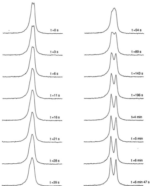
Figure 5.30: Spectra of PBLG acquired during relaxation following steady shear, applied for one minute at \dot{\gamma} = 0.08 \text{ s}^{-1} , in the 20^\circ cone and plate. The first spectrum, corresponding to t = 0 , was acquired immediately upon removal of the shear. The spectral width in all of the spectra is 1 kHz.
