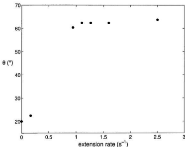
Figure 5.14: Director orientation \theta of liquid crystal polymer under extension in the four roll mill, plotted as a function of \dot{\mathcal{E}} . The critical extension rate \dot{\mathcal{E}}_c probably just exceeds 0.17 \text{ s}^{-1} .
