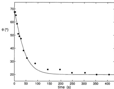
Figure 5.31: Fit of the Fréedericksz transition prediction to the NMR data for relaxation following shear at \dot{\gamma} = 0.08 \text{ s}^{-1} in the 20^\circ cone and plate. The fit yields 0.0293 = \chi_a B_0^2 / \mu_0 (\alpha_3 - \alpha_2) , or (\alpha_3 - \alpha_2) / \chi_a = 133 \times 10^7 \text{ Pa}\cdot\text{s} .
