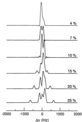
Figure 5.4: Spectra for different concentrations of PBLG in dioxane- d_8 , nitrobenzene- d_5 at 25°C in the quiescent state. The nematic phase is seen to set in at between 10% and 15%.
