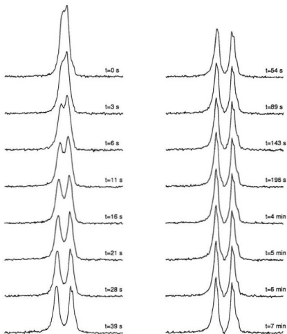
Figure 5.19: ^2\text{H} NMR spectra for relaxation of liquid crystal polymer following removal of 185.5 \text{ s}^{-1} shear in the vertical Couette cell. The width of each spectrum is 1 kHz. Within the 2 s required to acquire the first spectrum, the director has begun to relax from its orientation along the flow direction.
