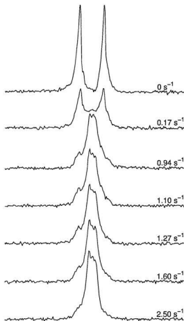
Figure 5.13: ^2\text{H} NMR spectra of PBLG as a function of rate of extension in the fourroll mill. The width of each spectrum here is 1 \text{ kHz} . The maximum splitting, exhibited in the zero extension spectrum, is 136.7 \text{ Hz} .
