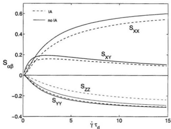
Figure 4.14: Solid lines are the S_{\alpha\beta} in the DE model without the independent alignment approximation. Dashed lines are curves calculated using IA.
