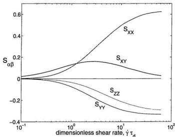
Figure 4.3: Predictions of the Doi-Edwards model for elements of the segmental alignment tensor S_{\alpha\beta} , as functions of shear rate made dimensionless by the reptation time \tau_d . The stress tensor \sigma_{\alpha\beta} is directly proportional to S_{\alpha\beta} . All of the calculations presented here were performed in Matlab [47].
