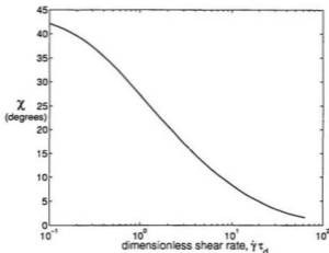
Figure 4.5: Prediction of the Doi Edwards model for the extinction angle \chi as a function of reduced shear rate \dot{\gamma}\tau_d .
