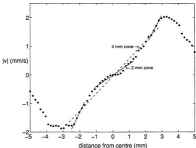
Figure 5.16: One-dimensional velocity profile along the extension axis in the four roll mill. The data corresponds to the middle row of the full NMR velocimetry image whose central region is shown in Fig. 5.15, for which the applied extension rate was 1.13 \text{ s}^{-1} . The solid line near the centre is the velocity gradient or slope averaged over the data points corresponding to the 2 mm region, from which the average local \dot{\mathcal{E}} is calculated to be 0.39 \text{ s}^{-1} . The dashed line indicates the slope over the 4 mm region, where \dot{\mathcal{E}} = 0.6 \text{ s}^{-1} . Also shown are straight line fits to the regions where the PBLG solution just emerges from between the rollers, where the calculated \dot{\mathcal{E}} is 1.1 \text{ s}^{-1} , much truer to the applied rate of extension.
