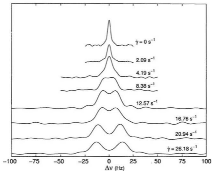
Figure 4.12: Spectra for S_{VY} , obtained with velocity gradient direction parallel to the magnetic field, at a range of shear rates for 610K PDMS melt containing the C_6D_6 probe at 10%.
