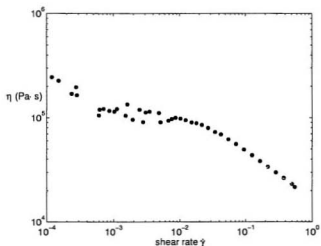
Figure 1.1: Representative flow curve, for 680K poly(dimethyl siloxane). The approximately constant viscosity at low shear rates (small deformations) but decreasing viscosity with shear rate at larger deformations is typical of polymeric liquids.
