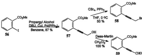
Scheme 4-16: Synthesis of 58 and 59
