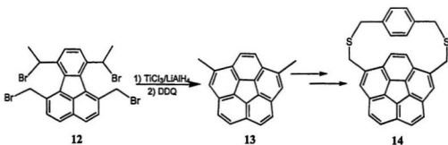
Scheme 3-8: Siegel's Synthesis of Corannulene Cyclophane 14.
