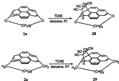
Scheme 6-5: Diels-Alder Adducts of Pyrenophanes and TCNE
