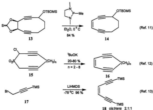
Scheme 4-3: More Syntheses of Eneidyne Moieties
