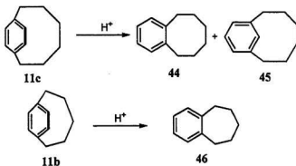
Scheme 2-13: Acid-Catalyzed Rearrangement of Paracyclophanes
