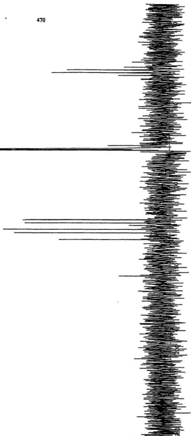
BB ^1\text{H} Decoupler OFF
