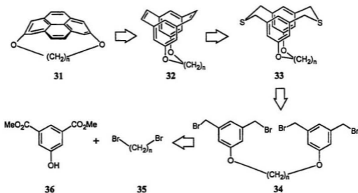
Figure 5-1: Retrosynthetic Analysis of 1,n-Dioxa[n](2,7)pyrenophane, 31
