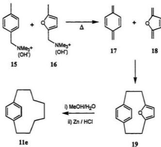
Scheme 2-3: p -Xylylene Route to [8]Paracyclophane
