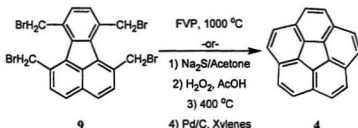
Scheme 3-5: Nonpyrolytic Synthesis of Corannulene
