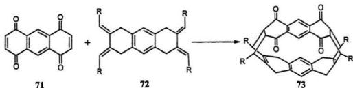
Scheme 3-27: Cory's Diels-Alder Route to Cyclocene Derivative 73
