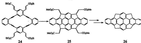
Scheme 4-6: Eneidyne-Cyclization Route to Dibenzopinakene Skeleton
