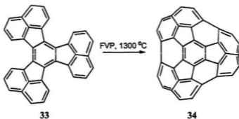
Scheme 3-15: Scott's Synthesis of 34
