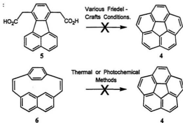
Scheme 3-3: Failed Corannulene Synthesis Attempts.
