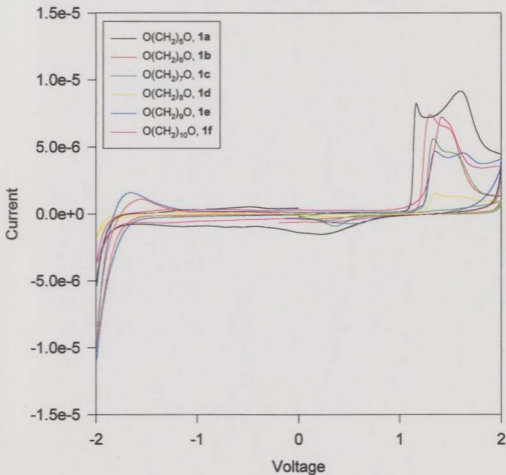
Figure 6-7: Dioxapyrenophane Cyclic Voltammetry, Normalized to 1 mM
