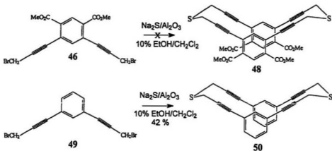
Scheme 4-12: Approaches to Expanded Thiacyclophanes
