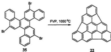
Scheme 3-16: Synthesis of 22 by Pyrolysis of Tribromoarene 35
