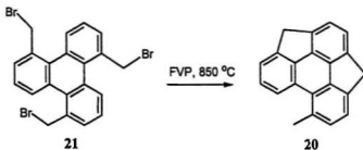
Scheme 3-11: Pyrolytic Dehydrobromination of 21 .
