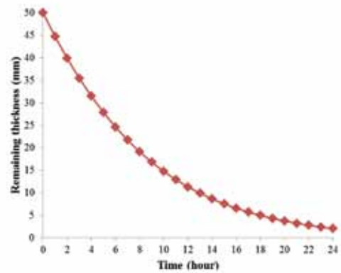
Figure 5: The change of slick thickness in the operational period.
