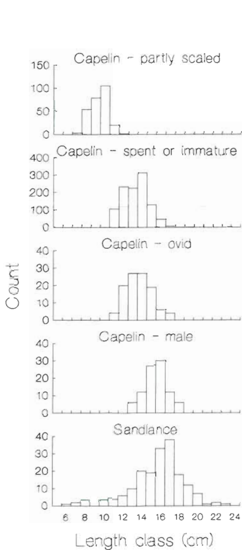
Fig. 4. Length distribution of larger fishes delivered to Atlantic puffin chicks on Great Island in 1992–94. Prey from mist-netted and telescopic samples and from loads dropped by puffins and recovered incidentally are included
