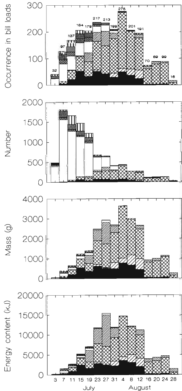
Fig. 7 Total prey delivered every 4 d throughout the nestling period to Atlantic puffin chicks on Great Island. Total prey includes all food delivered to 32 chicks that fledged and 15 that died. Numbers above bars in top: numbers of bill-loads recorded. For key to prey types, see Fig. 1
