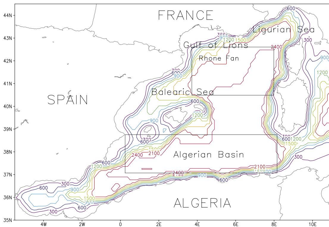
Figure 2. Bottom topography in the Algerian and Ligurian-Provençal basins. The two squared areas shown in the Gulf of Lions and the Algerian Basin are the areas, where energetic analysis is performed in section 6.
