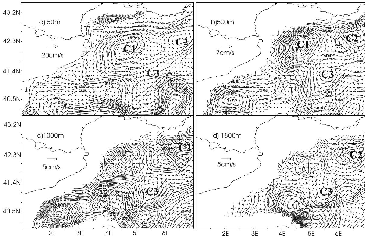
Figure 4. Mean velocity and density distributions in the Gulf of Lions for the period 1–3 January 1992 at (a) 50 m; (b) 500 m; (c) 1000 m; (d) 1800 m.
